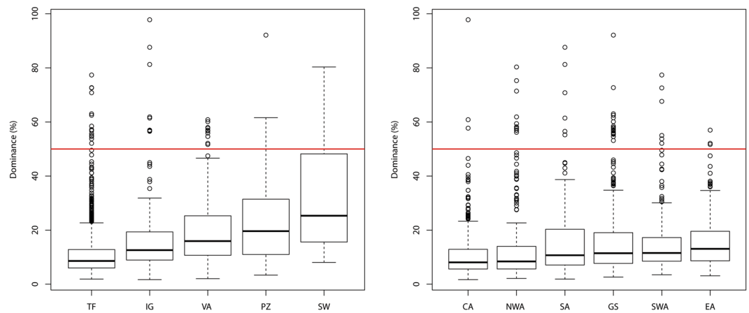
Figure 5. Percentage of dominance by plot (= relative abundance of the most abundant species of each plot) as a function of forest type (A) and region (B).
