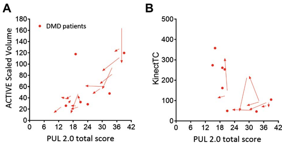
Fig. 6. ACTIVE and KinectTC change over time and relation with function tests. ACTIVE Scaled Volume plotted for baseline and 12 months follow-up of Duchenne muscular dystrophy (DMD) patients (red) against Performance of the Upper Limb (PUL) 2.0 total score in (A). Correlation was strong with PUL 2.0 ( \rho=0.76 ). ACTIVE Scaled Volume did decrease significantly over 12 months. KinectTC scaled trunk distance (trunk compensation in mm as a ratio to height in m) is plotted for baseline and 12 months follow-up of DMD patients against PUL 2.0 total score in (B). Correlation was moderate with PUL 2.0 ( \rho=-0.69 ).
