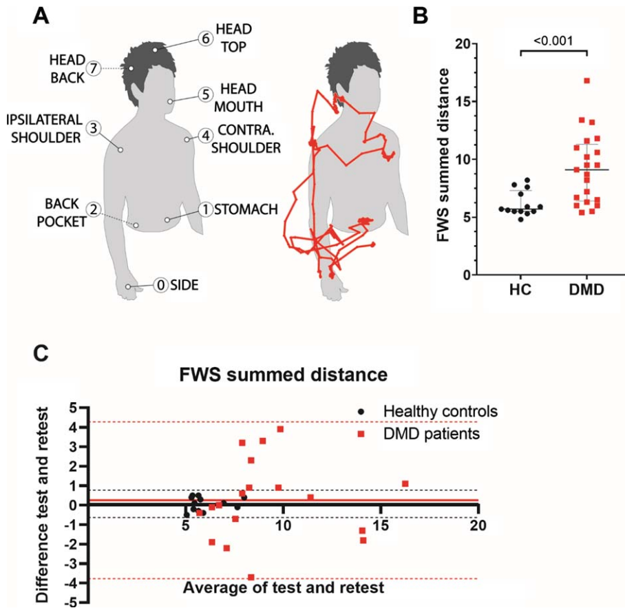
Fig. 3. Functional Workspace (FWS) summed distance setup, construct validity and reliability. In (A) the seven upper extremity targets of the FWS are shown and alongside this a typical movement pattern of the right wrist during the FWS is presented in red. Construct validity and reliability of the summed hand length distance to these seven targets are shown in (B) and (C) respectively. This summed distance differed significantly between Duchenne muscular dystrophy (DMD) patients and healthy controls (HC; p < 0.001 ). The Bland-Altman plot with mean bias (straight lines) and 95%-confidence intervals (dotted lines) shows that reliability is high for HCs (round), but much lower for patients (square). Average of the two trials is plotted on the x-axis and difference between the trials on the y-axis.
