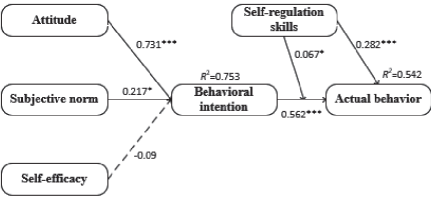
Fig. 4.2. Results of structural equation modeling.
