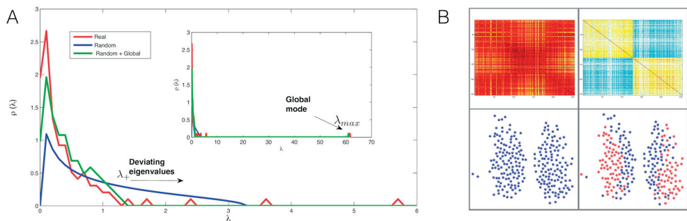
Figure 2. (A) Empirical eigenvalue density versus calculated eigenvalue density for the two random models. (B) The community structure of the SCN as resolved by our method. On the left, is the community structure detected by random model without filtering the global mode (Random). On the right, is the community structure detected by random model once the global mode is filtered (Random + Global). In the bottom panels are the partitions detected, where each community is marked with a different colour. In the top panels are the corresponding resolved filtered correlation matrices displaying the resolved structure as a block matrix.
