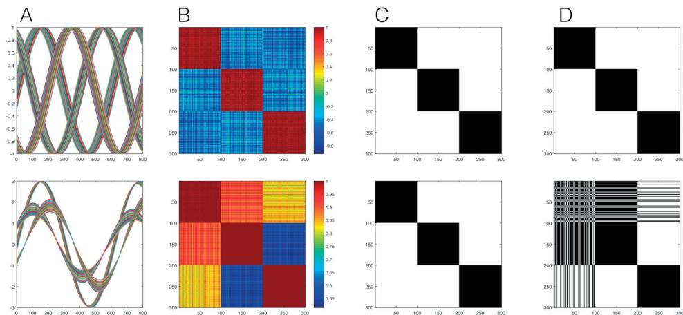
Figure 3. Illustration of misidentification due to the presence of common trends in a comparison between the method by Rubinov and Sporns (2011; based on a null model with independent entries of the correlation matrix) and our alternative approach (based on the more appropriate null model with dependent entries constructed from random matrix theory). (A top) 300 synthetically generated time series in a system with 3 modules, each containing 100 oscillating series with random phases, (A bottom) 300 synthetically generated time series as before, with a strong global periodic signal. (B) the corresponding correlation matrix, top and bottom accordingly, showing a clear block structure. The output of our method (C) and the Rubinov-Sporns method (D) in terms of likelihood matrices indicating the frequency with which two neurons are found in the same community in 1000 runs of both methods. We can see that the Rubinov-Sporns method is able to correctly separates the 3 modules in the more straightforward case of clear positive and negative correlation (D top). In the more complex case where the correlation are obscured by a strong common trend the Rubinov-Sporns method merges the first module with the other two clusters. Using the proper null model our method is able to correctly separates the 3 modules in both cases (C).
