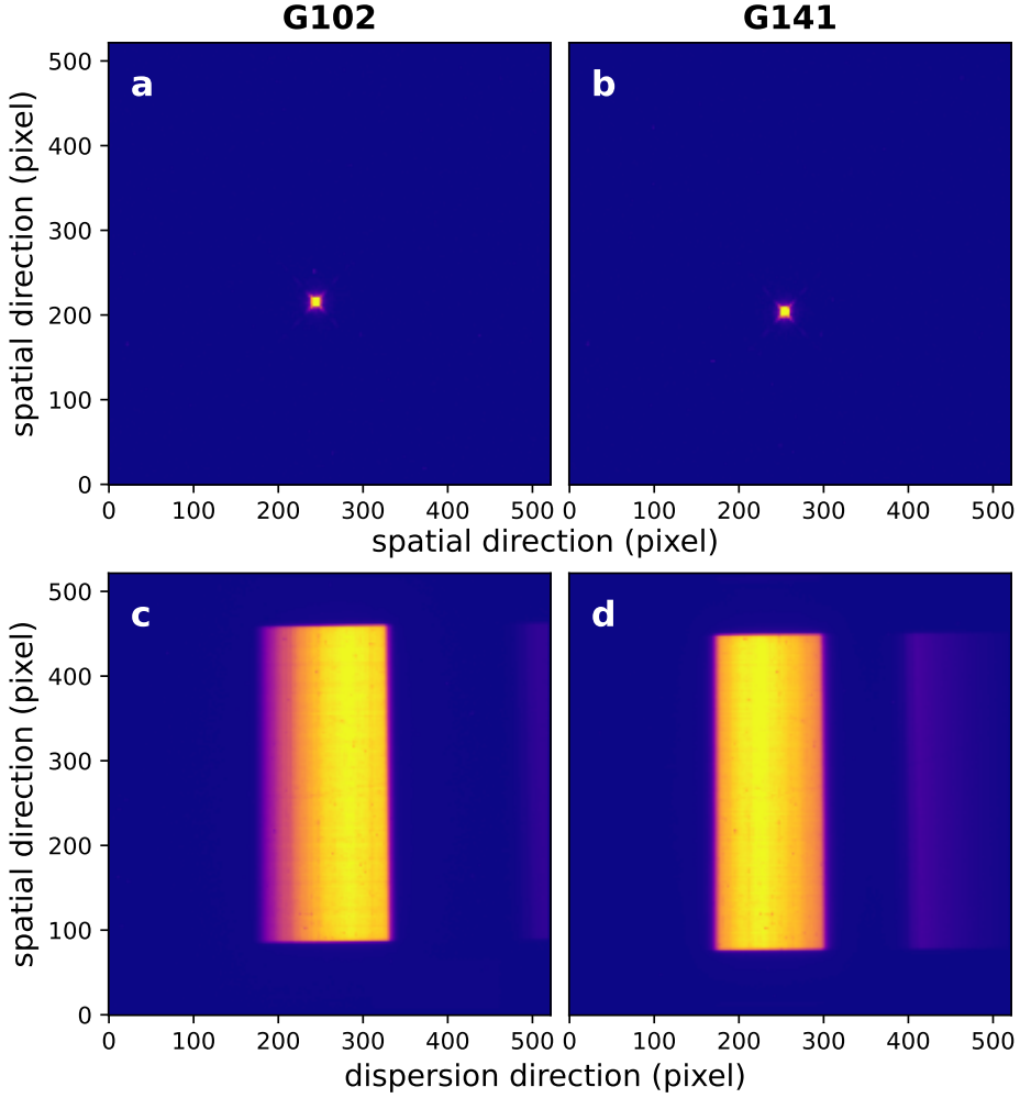
Figure 5.2: Examples of calibrated intermediate IR multiaccum image (IMA) files using the 512x512 subarray (SQ512SUB) on HST /WFC3. The top panels show the undispersed “direct images” of KELT-11 taken with the WFC3 F130N narrow-band filter for the G102 (panel a) and G141 (panel b) observations. The bottom panels c and d show first-order 2D spectra for the last up-the-ramp sample (i.e., the last non-destructive read) for a randomly chosen exposure in each observation. The faint second-order spectra (which are not used in this work) can be seen on the right side of the subarray.
