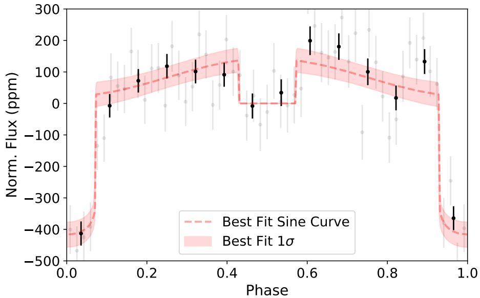
Figure 2.2: Phase curve of K2-141 b after phase folding the complete Spitzer observations. The eclipse is at phase = 0.5. The best fitting model shown in red describes the observed thermal emission from the planet as a sinusoidal function. Each bin in black (gray) consists out of 7200 (1800) Spitzer 2-second exposures. The pairs plot for this model can be found in the Appendix, Section 2.C.5.
