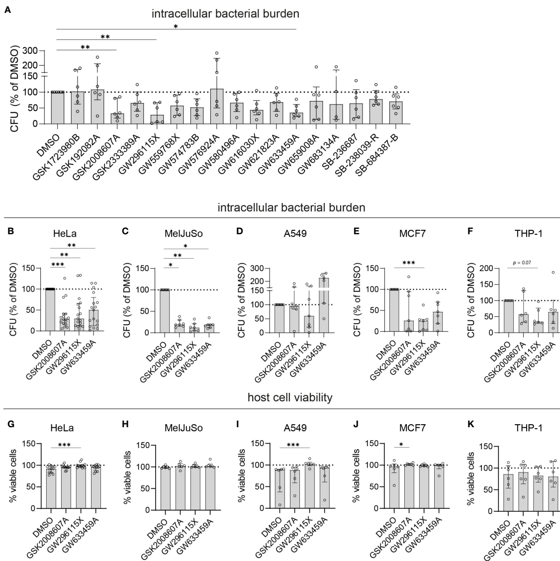
FIGURE 2 Validation of selected PK1S hit compounds. (A) The efficacy of the PK1S hit compounds against intracellular MRSA was determined by CFU count and given as the percentage of the DMSO control. (B–F) The efficacy of GSK2008607A, GW296115X and GW633459 on the bacterial burden of MRSA-infected HeLa cells (B, n=17), MelJuSo cells (C, n=7), A549 cells (D, n=7), MCF7 cells (E, n=7) and PMA-differentiated THP-1 cells (F, n=6) was determined by CFU count. (G–K) The effect of the compounds on cell viability was assessed using LDH-release assay for HeLa cells (G), MelJuSo cells (H), A549 cells (I), MCF7 cells (J) and PMA-differentiated THP-1 cells (K). Bars and error bars show the median ± interquartile range. Each datapoint represents the results of an independent experiment. Statistical significance of observed differences was tested in comparison to the DMSO controls using Friedman tests (* p < 0.05; ** p < 0.01; *** p < 0.001).
