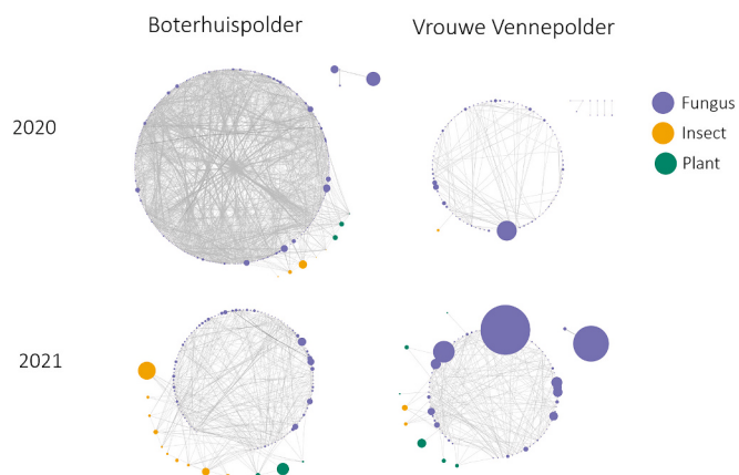
Fig. 4. Connectedness of species networks in the in the Boterhuispolder (reference site) and the Vrouwe Vennepolder (focal site, in transition) for two years. The total number of taxa determines the size of the network and the size of the nodes marks the average abundance of the organisms across the plots in that polder and the color the identity of the organism. Purple marks fungi identified as amplicon sequence variants (ASV)s, green color marks plants, yellow indicates insects. (For interpretation of the references to color in this figure legend, the reader is referred to the web version of this article.)
