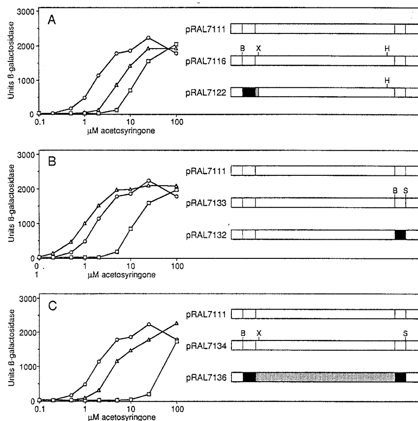
Fig. 1. Induction characteristics of virA-tar chimeric genes in Agrobacterium . The vir gene induction response of LBA2524 harbouring a wild-type virA gene (○), a virA gene containing several restriction sites (△) or the virA-tar chimeric genes (□) was tested in induction medium with 10 mM glucose and various concentrations of acetosyringone. Flasks were shaken for 18 h at 28 °C and units β-galactosidase were determined as described [20]. Open bars represent coding regions of virA , black and stippled bars represent coding regions of tar . The restriction sites Bss HII (B); Xba I (X); Hpa I (H) and Sal I (S) shown were used for the construction of the different virA-tar gene fusions.
