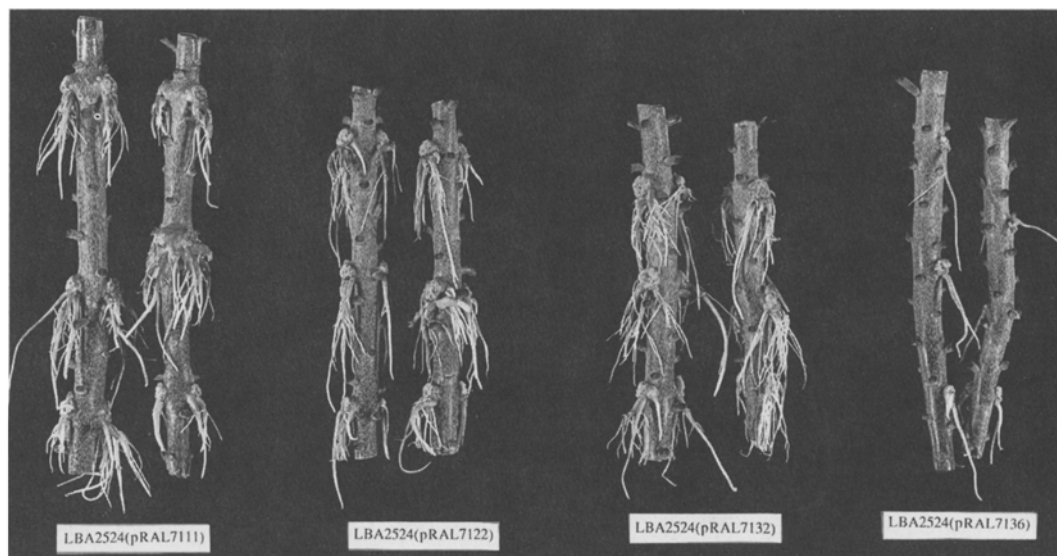
Fig. 2. Tumour response of the virA-tar chimeric genes in Agrobacterium tumefaciens strain LBA2524 upon infection on stems of Kalanchoe tubiflora . Tumour formation was evaluated after 3 weeks.
