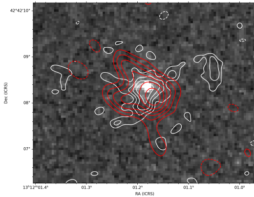
Figure 2.9: HST-NICMOS F160W-band image with CO(1-0) (white) and CO(6-5) (red) contours overlaid on top. Contours start at \pm 2\sigma and increase in steps of \sigma = 4.4 and 93.8 \mu\text{Jy beam}^{-1} \text{ km s}^{-1} . The beam sizes are 0.39'' and 0.6'' for CO(1-0) and CO(6-5), respectively. The stellar emission is concentrated and its peak is coincident with the CO(1-0) and CO(6-5) emission peaks. CO(6-5) emission is equally extended as CO(1-0), and its semi major axis appears to be almost perpendicular to that of CO(1-0).
