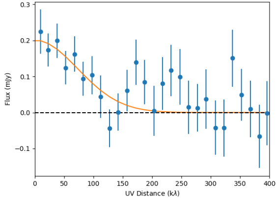
Figure 2.4: Visibilities (uv)-profile of J13120. The uv-data were extracted from the channels within the full-width at zero intensity of the line from the cube and averaged in bins of 15 k \lambda . We fit the profile with a single Gaussian to estimate the intrinsic source size, finding a half-light radius of 1.20 \pm 0.15 arcseconds, consistent with the 2D elliptical Gaussian fit to the 0th moment map.
