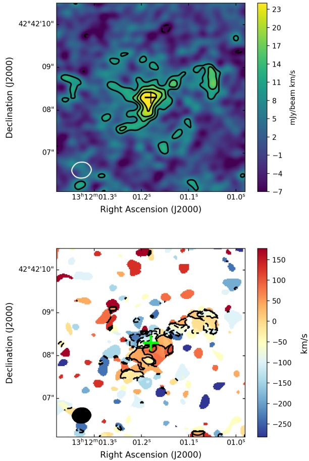
Figure 2.3: CO(1-0) 0th (top) and 1st (bottom) moment map of SMM J13120 at a resolution of 0.39'' . The 0th moment map contours start at \pm 2\sigma and increase in steps of \sigma = 4.4 \text{ mJy km s}^{-1} . The 1st moment map was clipped at 2 times the rms noise per channel ( \sigma = 9 \mu\text{Jy beam}^{-1} ), and contours are shown in steps of 50 \text{ km s}^{-1} . We fit a 2D elliptical Gaussian to the 0th moment map to determine the peak position of the emission, shown by the cross, corresponding to the white cross in Fig. 2.2.
