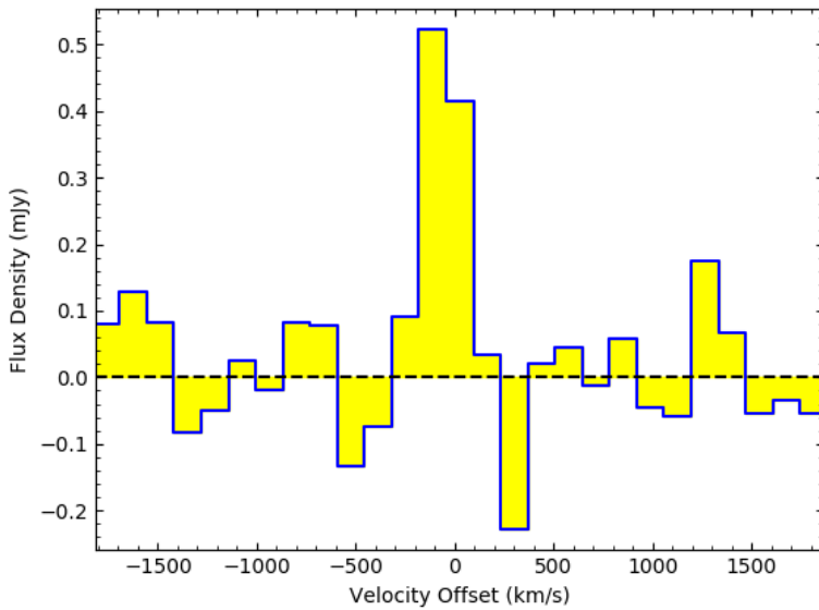
Figure 2.10: CO(1-0) spectrum of SMM J13120 with a spectral resolution of 138 \text{ km s}^{-1} . No evidence for a broad ( \sim 1000 \text{ km s}^{-1} ) line is seen in the deeper multi-configuration data.
