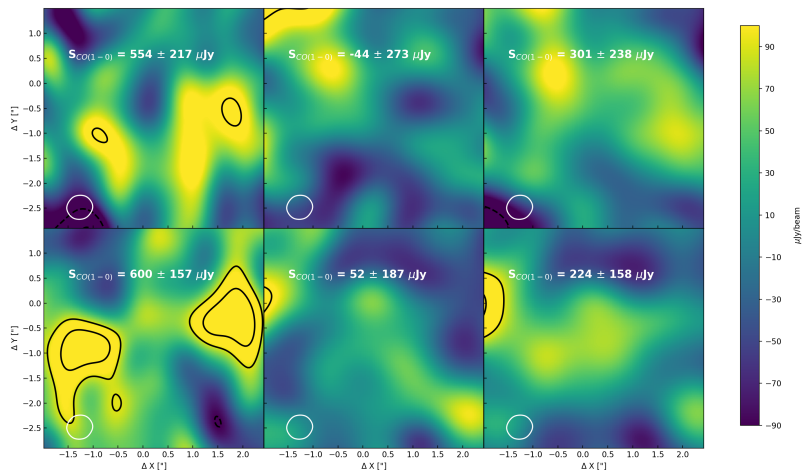
Figure 2.12: 0th moment maps collapsed over the negative and positive velocity offsets where emission was present in the spectrum in R11. The top and bottom rows show the emission at negative ( -800 to -600 \text{km s}^{-1} ) and positive ( 400 to 600 \text{km s}^{-1} ) velocity offsets, respectively. The first, second and third column correspond to the earlier VLA dataset (R11), the new dataset presented here and the concatenated data, respectively. The flux density was extracted from the same circular aperture. The new and concatenated datasets do not show emission above the 2\sigma noise, and the flux density is consistent with the earlier VLA data within the errors, highlighting the uncertainty in the original dataset.
