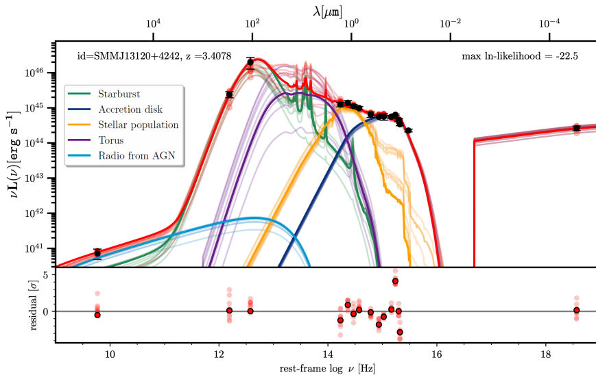
Figure 2.5: SED modelling of the radio-to-X-ray photometry available for J13120 using the Bayesian SED-fitting code AGNfitter-rX (Calistro-Rivera+16, Martinez-Ramirez, in prep.). In the main panel the photometric data points are shown with black error bars. The best fit and ten realisations of the posterior distributions of the fit are drawn as coloured solid and transparent lines, respectively. The realisations display the uncertainties associated with the fits. The different colours represent the total SED (red lines), the accretion disk and X-ray corona emission (dark blue), the host galaxy emission (yellow), the torus emission (purple), the galactic cold dust emission and radio emission that originates in star formation (green) and the radio AGN emission (turquoise). The lower panels show the residuals expressed in terms of significance given the data noise level for the best fit and the 10 realisations.
