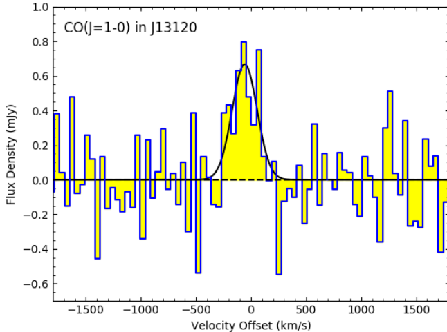
Figure 2.1: CO(1-0) spectrum of SMM J13120 with a spectral resolution of 46 \text{ km s}^{-1} . The solid line shows the Gaussian fit to the data, which yields a peak flux density of 0.67 \pm 0.14 \text{ mJy} and a FWHM of 267 \pm 64 \text{ km s}^{-1} .
