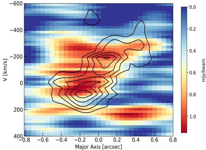
Figure 2.7: PV diagram of CO(6-5) emission in J13120 extracted from an axis with PA = 42.7°. Black contours correspond to the CO(1-0) PV diagram extracted from the same axis (see Figure 2.6). The CO(6-5) emission shows evidence for a similar gradient as seen in CO(1-0).
