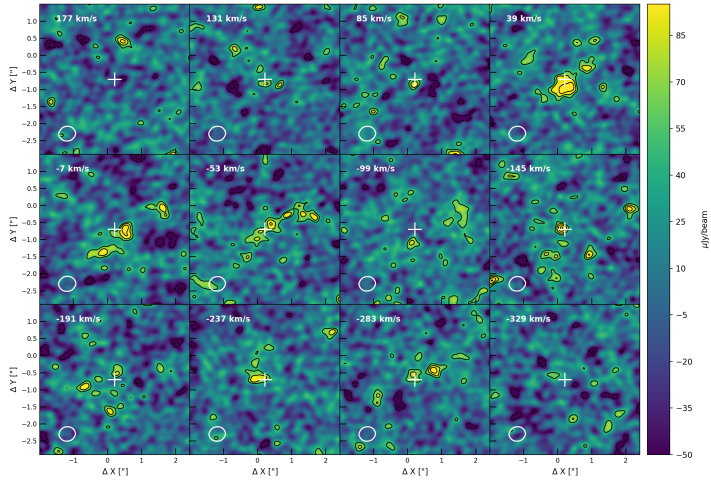
Figure 2.2: CO(1-0) emission maps in SMM J13120 in 46 \text{ km s}^{-1} channels. Cleaned maps are shown at native resolution of 0.39'' from 177 \text{ km/s} in the top left channel to -329 \text{ km/s} in the bottom right. The shape of the beam is displayed in each channel. The white cross corresponds to the best fit peak position of a 2D elliptical Gaussian to the 0th moment map. Contours start at \pm 2\sigma and increase in steps of \sigma = 27.7 \mu\text{Jy beam}^{-1} .
