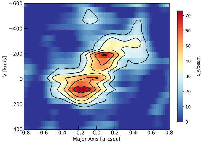
Figure 2.6: Position-velocity (PV) diagram of CO(1-0) emission in J13120. The axis of extraction is at PA of 42.7^\circ and an aperture of 0.3'' was used. Despite the disturbed velocity field seen in Fig. 2.3, bottom, there is a clear velocity gradient in SMM J13120.
