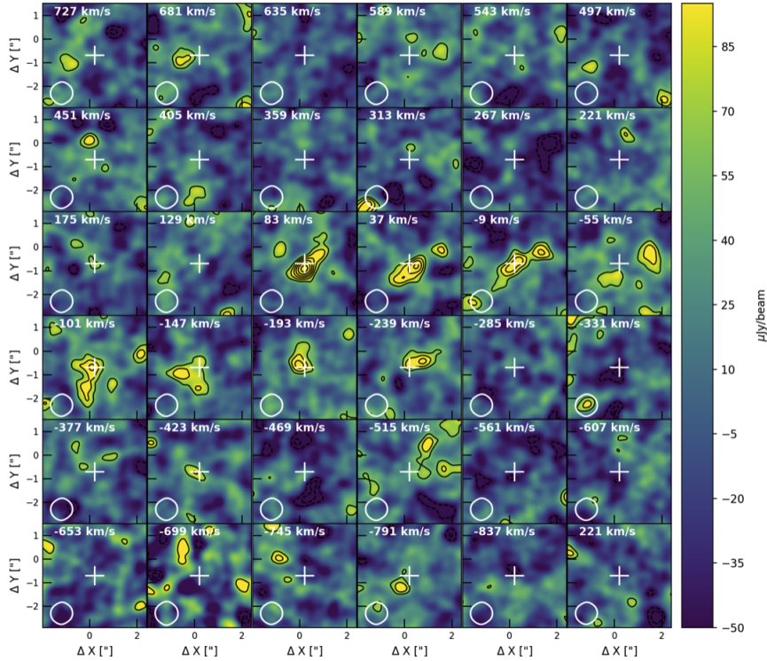
Figure 2.11: CO(1-0) emission maps in SMM J13120 in 46 \text{ km s}^{-1} channels. The data was tapered to a resolution of 0.94'' to search for faint extended emission that could have been missed at higher resolution. The shape of the beam is displayed in each channel. The white cross corresponds to the best fit peak position of a 2D elliptical Gaussian to the 0th moment map. Contours start at \pm 2\sigma and increase in steps of \sigma = 35 \mu\text{Jy beam}^{-1} .
