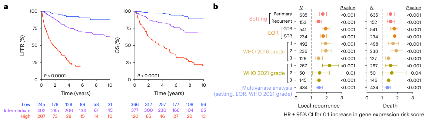
Fig. 2 | Gene expression biomarker discrimination of meningioma outcomes.
