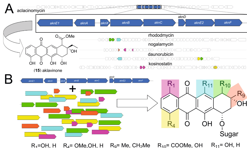
Figure 15. Generation of hybrid anthracyclines in S. galileus producing aclinomycins. (A) The aclinomycin BGC results in the formation of aklavinone (15). This aglycone is not modified by native tailoring enzymes, and therefore cloning of tailoring genes from the rhodomyacin, nogalamycin, daunorubicin and kosinostatin pathways has led to formation of novel hybrid compounds. (B) Libraries of anthracyclines have been generated through modification of the aglycone at R 1 (magenta), R 4 (yellow), R 9 (orange), R 10 (green), and R 11 (cyan).
