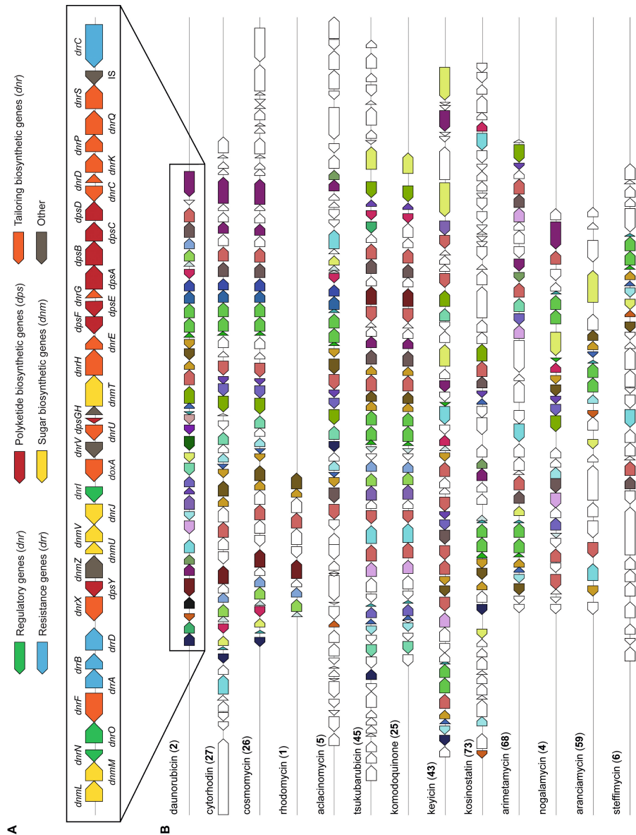
Figure 14. Currently known anthracycline biosynthetic gene clusters. (A) Schematic representation of the daunorubicin BGC. The color scheme represents the global gene function, classified as regulatory genes (green), resistance genes (blue), polyketide biosynthetic genes (red), sugar biosynthetic genes (yellow), tailoring genes (orange), or other (grey). (B) Gene cluster homology search of the daunorubicin BGC against twelve other experimentally verified anthracycline BGCs using MultiGeneBlast (v1.1.13) with default parameters 21,2 . The daunorubicin BGC is visualized in a color scheme that represents homology between genes of different clusters. For most BGCs the total extent of the clusters is unclear. Note that the aranciamycin and steffimycin BGCs lack sugar biosynthesis genes. The rhodomycin BGC has been sequenced only partially.
