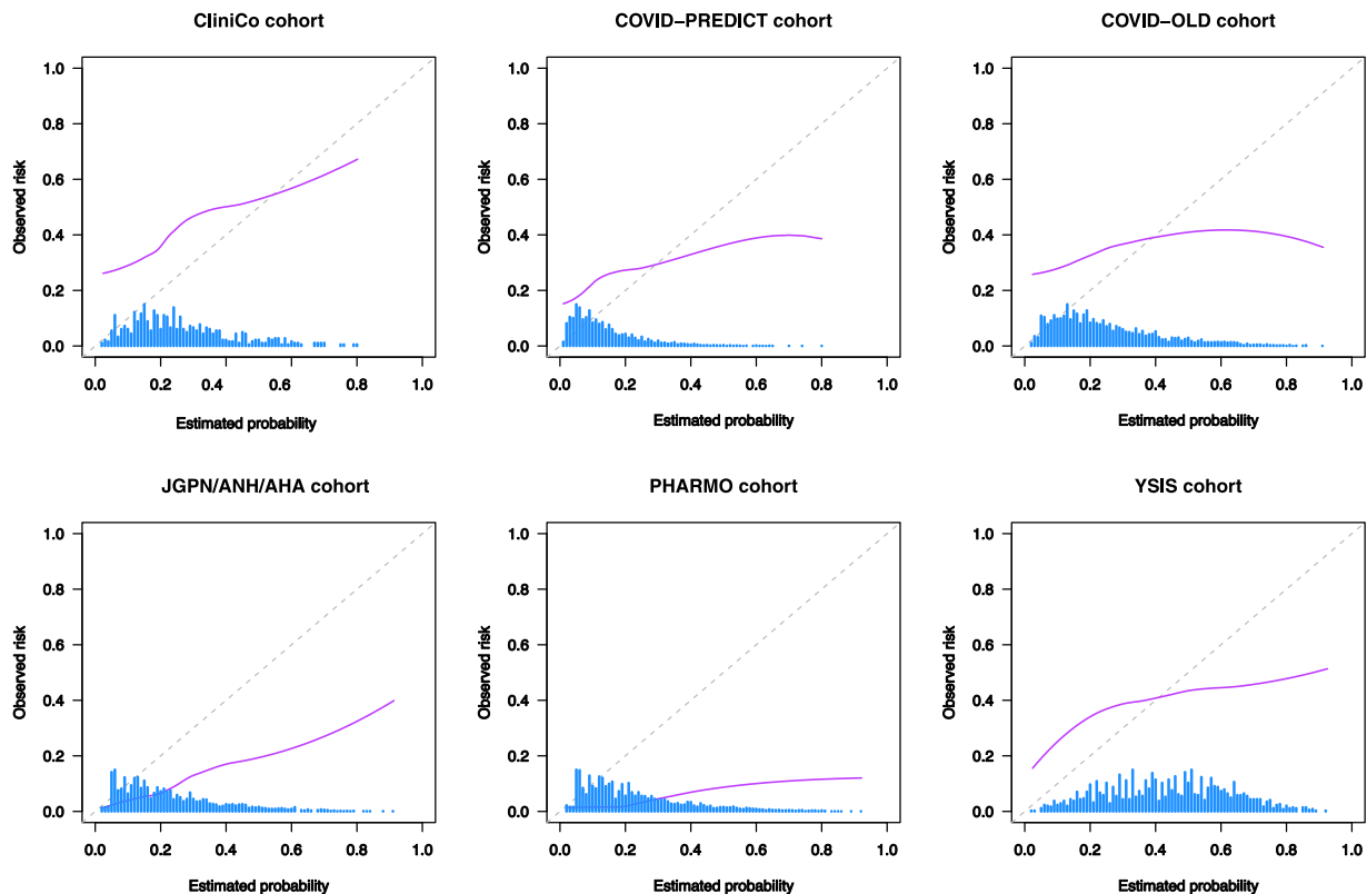
Fig. 3. Predictive performance of the GAL COVID-19 mortality model in all validation cohort in 2020 (Calibration is shown using locally weighted).
