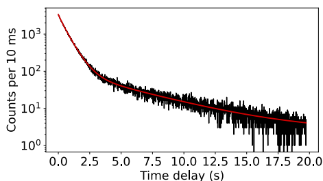
Figure 3.6.: Phosphorescence decay curve of dibenzothiophene crystals at 2 K. The integration time is 10 ms per point, measured in the spectral region determined by a band pass filter between 440-460 nm. The red curve is a fit by a sum of three exponential decays.
