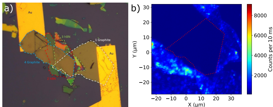
Figure 5.28.: a) Microscope image of the heterostructure with at the bottom a layer of graphite in contact with one of the gold electrodes. Followed by two hBN flakes on top of each other, with molecules deposited in between and a top graphite layer connected to the other electrode. Panel (b) shows the fluorescence image of the region where all layers overlap, bordered with a red dashed line. The fluorescence signal in this region is very weak, which is possibly due to the low transparency of the top graphene layer. See also the low contrast on the left electrode in (a), where the top graphene layer overlaps with the highly-reflecting gold.
