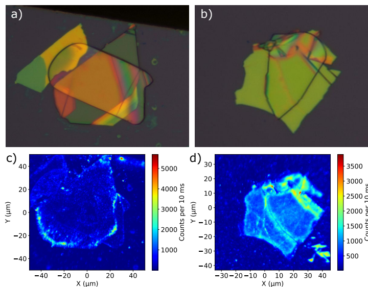
Figure 5.26.: Examples of encapsulation of an hBN flake by another flake of hBN, by the stamping method. In panel (a) the bottom hBN was not annealed and in panel (b) the bottom hBN was annealed. In both cases, molecules were deposited by sublimation before encapsulation (and annealing). The corresponding fluorescence maps of the flakes in (a) and (b) are respectively shown in panel (c) and (d). Note that the background is much higher for the annealed flake (d) compared to the non-annealed flake in (c). Hundreds of terrylene molecules were found on the non-annealed flake, while only a single terrylene molecule was found on the annealed flake.
