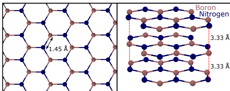
Figure 5.1.: Structure of hexagonal boron-nitride. Boron and nitrogen are alternately arranged, with an interatomic distance of 1.45 Å. In multilayer hBN, the layers stack such that a nitrogen atom faces a boron atom and vice versa. The interlayer distance is 3.33 Å, which is the same as for graphene. 4
