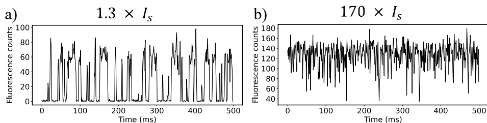
Figure 2.11.: Fluorescence time traces of molecule M1 over a time span of 500 ms, with a 1 ms integration time per point. A significant change in blinking dynamics can be observed between panel (a) representing a low excitation intensity and panel (b) a high excitation intensity. The reduction in dark times can be explained by a change in the triplet lifetime due to reverse intersystem crossing.
