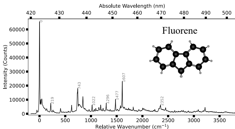
Figure 3.7.: Phosphorescence spectrum of an impurity of dibenzothiophene. Note that the structure of the spectrum is very similar to that of dibenzothiophene. Hence, this is likely a molecule with a related chemical structure. In fact, the vibrational fingerprint matches that of fluorene. 7 The structure of fluorene is shown on the top right. Compared to dibenzothiophene, the central sulfur atom has been replaced with a carbon atom, terminated with two out of plane hydrogen atoms.
