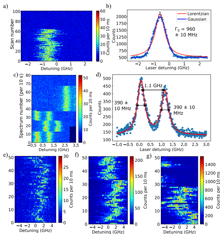
Figure 5.17.: (a) Series of excitation spectra of a molecule at 581.96 nm, taken with 11 W/cm 2 laser intensity. (b) The summed intensity of all the spectra in (a) builds up the figure. The excitation spectrum is fitted with both a Lorentzian and Gaussian distribution. The Gaussian distribution fits best and yields the indicated linewidth. (c) One of the narrowest resonances that are found on hBN is shown in this series of excitation spectra. (d) A fit of two Lorentzian distributions for the two resonance lines present in (c). (e), (f), (g) Spectral diffusion of a molecule recorded at increasing excitation intensities of 1 W/cm 2 in (e), 14 W/cm 2 in (f) and 250 W/cm 2 in (g).
