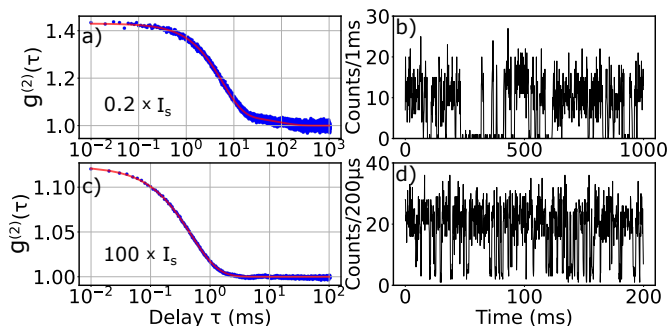
Figure 2.12.: Fits of the autocorrelation curves (left) and parts of the corresponding fluorescence time traces (right) of molecule M1 at a low excitation intensity of 20% of the saturation intensity in panel (a) and panel (b) and 100 times the saturation intensity in panel (c) and (d). Note that the time scales in (a) and (c) differ, while also the integration time for (b) is 1 ms and 200 \mu s for (d). In addition, the fit in (a) is a sum of two exponentials, while (c) was fitted to a single exponential decay.
