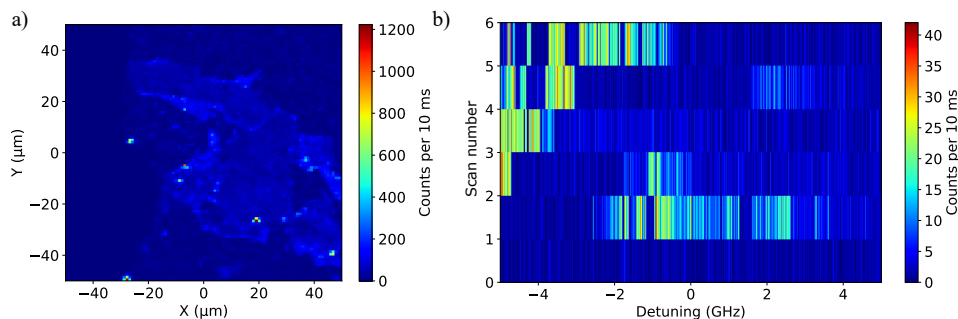
Figure 5.16.: a) Confocal fluorescence map of a collection of hBN flakes, taken at an excitation wavelength of 582.38 nm at a relatively high laser intensity of 350 \text{ W/cm}^2 . The brightest spot, around (X = 20, Y = -25) corresponds to the emission of the molecule in Figure 5.18. b) Common behavior of a molecule shown in a series of excitation spectra. The series of spectra were taken with the procedure mentioned in the text. In the second line of the scan, the laser was pointed to the position of the molecule. The strong spectral diffusion and blinking makes it difficult to extract a linewidth from this measurement.
