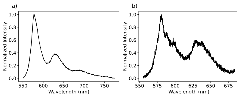
Figure 5.8.: Fluorescence emission spectra of terrylene at room temperature. The spectrum in (a) is likely from an ensemble of terrylene molecules, while the spectrum in (b) might be from a single molecule, as the emission was relatively isolated.
