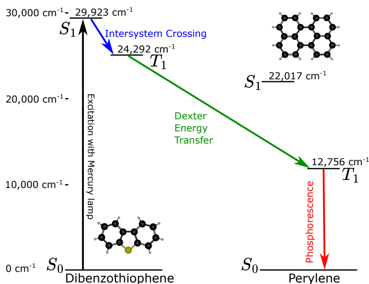
Figure 3.1.: Energy level scheme of perylene-d12 in dibenzothiophene. The energy levels of dibenzothiophene are known from the literature 1 The S_0 - S_1 energy gap of perylene-d12 was derived from the emission spectrum in Figure 2.4 of Chapter 2 and the S_0 - T_1 energy gap is derived from the phosphorescence spectrum in the present chapter. The excitation scheme relies on a UV excitation ( < 334 nm) of the singlet excited state of dibenzothiophene, followed by an intersystem crossing to the triplet state of dibenzothiophene. The excitonic energy may then be transferred to perylene through Dexter energy transfer, where upon the excited triplet of perylene may release a phosphorescence photon.
