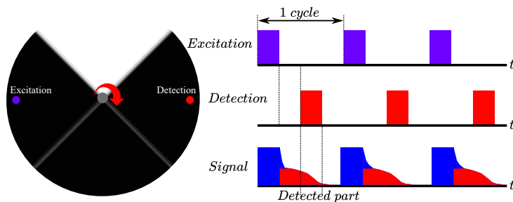
Figure 3.2.: Schematic of the optical chopper scheme. The excitation and detection beam are located at opposite sides of the chopper, which has an open part over a quarter of its area. The rotating chopper makes sure there is a delay of about \frac{1}{4} of a full rotation between the excitation and detection windows to remove unwanted short-lived photoluminescence, in particular fluorescence. The excitation and detection cycles are shown in a square wave profile on the right. The signal, shown schematically in blue for fluorescence and red for phosphorescence is strongly exaggerated in terms of timescales, as the fluorescence decays six orders of magnitude faster than the phosphorescence of perylene.
