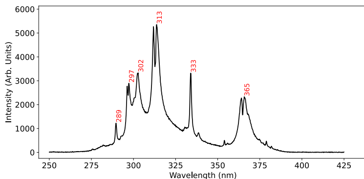
Figure 3.3.: Spectral lines of the mercury lamp that were transmitted by the filter that was used at the excitation side (FSR-U340). All the spectral lines below approximately 334 nm are used for the S_0 \rightarrow S_1 transition of dibenzothiophene. The spectral lines above 334 nm could still excite the much weaker S_0 \rightarrow T_1 transition of dibenzothiophene.
