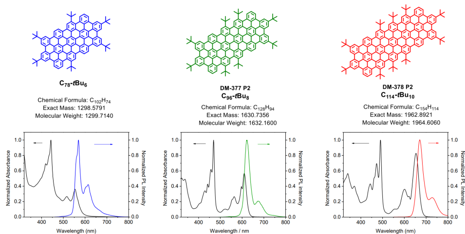
Figure 5.21.: Shown on the top are the chemical structures of the three graphene quantum dots with below their corresponding absorption (black) and fluorescence emission spectra (in color). The image was provided to us by the group of prof. J.S. Lauret from Paris Saclay university. The spectra were measured with 1,2,4-trichlorobenzene as the solvent.
