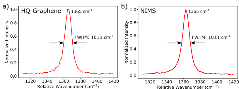
Figure 5.6.: Spectra of the inelastically-scattered light from a multilayer hBN flake (from supplier HQ Graphene in panel (a) and NIMS in panel (b)), taken with a 532 nm laser. The single Raman peak observed for both cases at 1365 cm -1 , with a FWHM of 10 ± 1 cm -1 , was taken at a resolution of around 1-2 cm -1 . The spectrum is recorded at room temperature with a 1200 lines/mm grating and a 0.1 mm slit size.
