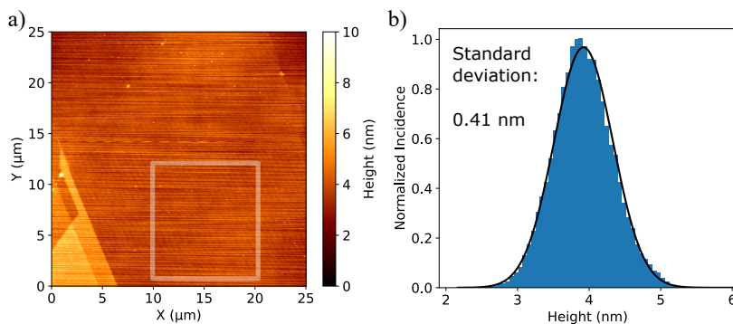
Figure 5.5.: AFM scan of a flat area of an annealed hBN flake (500 °C for 12 hours). The white rectangle encloses the region that builds up the histogram in b). The Gaussian distribution of surface heights shows a standard deviation of 0.41 nm. Tilts and drifts in the scan have been subtracted by a line-by-line linear fit.
