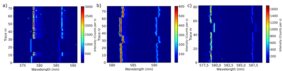
Figure 5.27.: Series of emission spectra of encapsulated molecules. The molecule in panel (a) was located in the encapsulated part of the annealed bottom flake. It was also the only molecule that we could find on this sample. Panel (b) and panel (c) show examples of spectral diffusion that we observed for molecules that were located on the non-annealed hBN flake, inside the encapsulated region.
