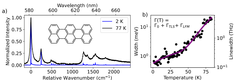
Figure 5.9.: Emission spectra of a single terrylene molecule around 582 nm, taken at two temperatures, 2 K (blue) and 77 K (black). Both spectra have been normalized to unity relative to the intensity of the 0-0 ZPL. b) Linewidth of the 0-0 ZPL of a single terrylene molecule (not the one shown in (a)). The linewidth was fitted to the equation in inset, where \Gamma_{TLS} scales linearly with temperature and \Gamma_{LFM} is given by the Arrhenius law, described in equation 5.1. The linewidth at the lowest temperature was limited by the spectrometer resolution ( 1.7 \pm 0.1 \text{ cm}^{-1} ). A zoomed-in version of the spectrum in (a) can be found in Figure 5.11b.
