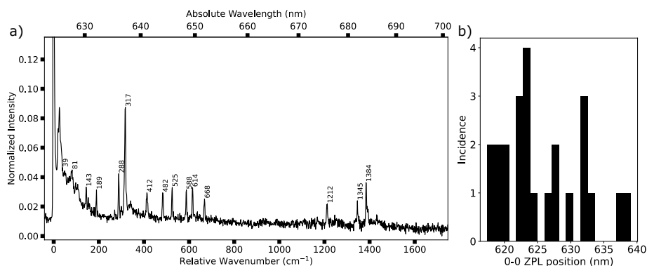
Figure 5.20.: (a) Fluorescence emission spectrum of molecule X with annotated vibrational peaks, normalized to the intensity of the 0-0 ZPL. The excitation frequency was 532 nm. (b) Histogram of the location of the 0-0 ZPL of 24 molecules that shared the vibrational fingerprint as in (a).
