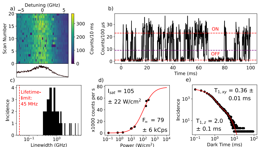
Figure 5.18.: a) Excitation spectrum of the 0-0 ZPL of a single molecule that did not jump out of resonance with the laser, even at higher excitation intensities. The homogeneous linewidth is about 4.7 \pm 0.3 \text{ GHz} and is measured with a scan rate of 5 seconds per row. The line plot underneath the figure shows the asymmetric profile of the 0-0 ZPL. A time trace of the fluorescence signal of this molecule in (b) shows characteristic quantum jumps due to intersystem crossing to the triplet state. However, in some cases the molecule remained dark for much longer times than the triplet lifetime, as is also visible in (a). These long dark times may be attributed to a relatively short spectral jump back and forth between another (out-of-range) spectral position. The purple line represents the threshold set between the ON and OFF state of the fluorescence. c) Distribution of 0-0 ZPLs linewidths found for molecules on different flakes. The red dashed vertical line represents the lower limit set by the fluorescence lifetime. Due to the large distribution of linewidths, the horizontal axis has been set to a logarithmic scale. d) Saturation curve of the fluorescence of the molecule in (a), fitted with F(I) = F_{\infty}(I/I_s)/(1 + I/I_s) , where I_s is the saturation intensity of the laser and F_{\infty} is the maximum fluorescence rate. The saturation intensity is 105 \pm 22 \text{ W}/\text{cm}^2 , 2 orders of magnitude larger than typically obtained with our setup for near-lifetime-limited emitters. This is explained by the 2 orders of magnitude broader linewidth, as the saturation intensity scales linearly with the linewidth of the transition. e) Distribution of dark periods in the resonance fluorescence signal, recorded over 60 s with 100 \mu s time bins (as in (b)). The characteristic timescales of the fit (red curve) are shown on the top right and bottom left.
