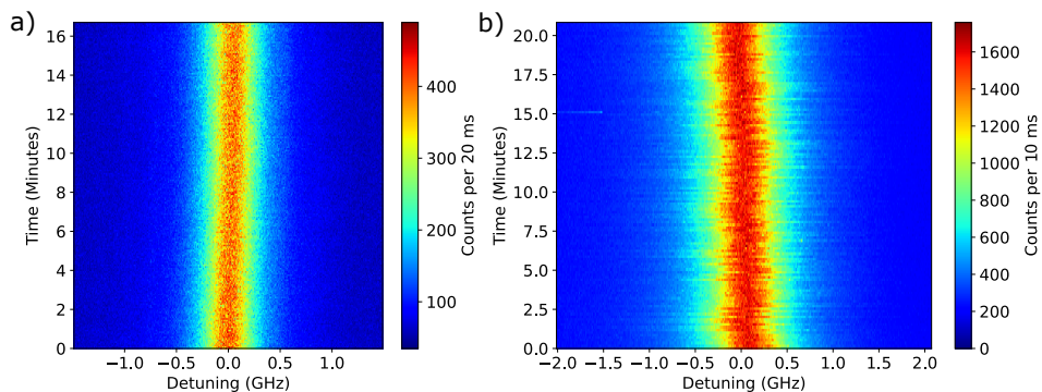
Figure 6.7.: Examples of time traces of excitation spectra, taken at high excitation intensities. The colors in the heatmap are relatively uniform due to shortened shelving in the triplet state. The molecule in panel (a) has a linewidth broadened to 496 MHz, at about 100 times saturation intensity. The molecule in panel (b) has a linewidth of 770 MHz, at about 225 times the saturation intensity. This molecule has a particularly uniform color in the excitation spectra, given that the integration time is only 10 ms and indicates very short dwell times in the triplet state. With the highest excitation intensity available, we could reduce triplet lifetimes down to 60 \mu s.
