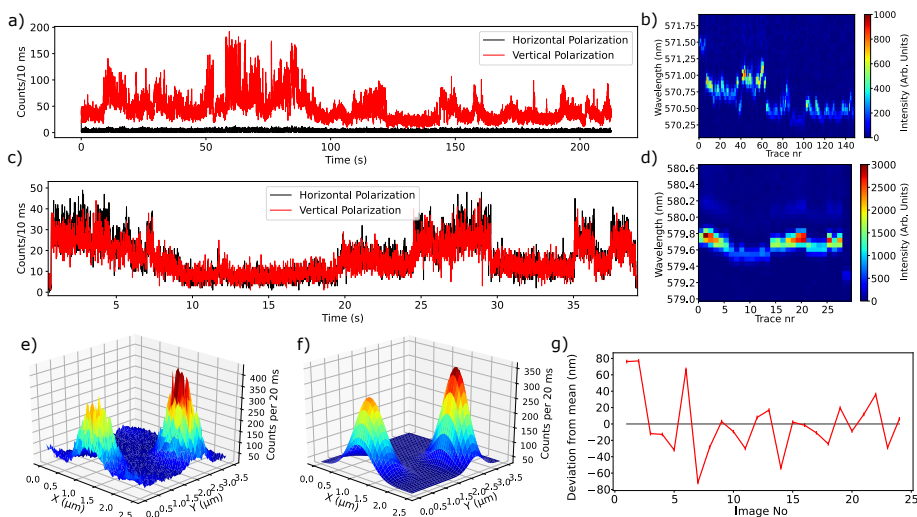
Figure 5.15.: a,b) Fluorescence time trace and spectra of a molecule whose fluorescence is nearly perfectly oriented with the vertical polarization component. Spectral jumps during the time trace have no influence on the horizontal polarization component. c,d) Shows the time trace and spectra of another molecule with comparable intensities in both polarization channels. Also here the spectral jumps have no influence on the ratio of the two polarization components. Around 28 s, the molecule jumps to a spectral position where the excitation was much less efficient, the signal dropped considerably, and therefore the data was cut here. The spectra in b) and d) were recorded with a 1 s integration time. The time scales of the fluorescence time trace and of the spectra are different, due to some delay between the recorded spectra. Panel (e) and (f) show respectively the experimental and fitted point-spread functions of two molecules that are approximately 2 \mu\text{m} apart from each other and do not (or barely do) overlap with the PSFs from other molecules. A single scan consisted of 100 \times 100 pixels over a range of 5 \times 5 \mu\text{m}^2 and took about 200 s to acquire with the scanning mirror. In total, 24 of these images were acquired over the course of 90 minutes with short pauses in between. Panel (g) shows the distance between the two molecules extracted from 24 consecutive confocal images, as in panel (e). The average error of the fit is just a few nm, but the measurements likely have a larger error due to spectral jumps occurring while recording the PSF. For all fitted data, the distance appears to revert around a mean value of 2.18 \mu\text{m} , and shows no clear trend. Hence, if there is any spatial diffusion, its extent is very limited.
