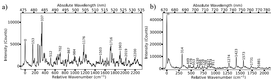
Figure 3.8.: Phosphorescence spectra of unidentified impurities in dibenzothiophene. Panel (a) shows a phosphorescence spectrum of an impurity found in the experiment where we detected perylene-d12 phosphorescence as well. The spectrum is very crowded with lines and might be mixed with another impurity. Panel (b): Apart from perylene-d12, this was the most red-shifted impurity found. The spectrum is different in shape and crowdedness compared to the spectrum of dibenzothiophene in Figure 3.5, the spectrum of fluorene in Figure 3.7 or the spectrum in (a), but resembles more closely a spectrum of a general aromatic compound, without heteroatoms. Unfortunately, the tail of this spectrum stretched all the way into the region of the phosphorescence of perylene-d12, which made this sample useless for the detection of the perylene-d12 triplet energy.
