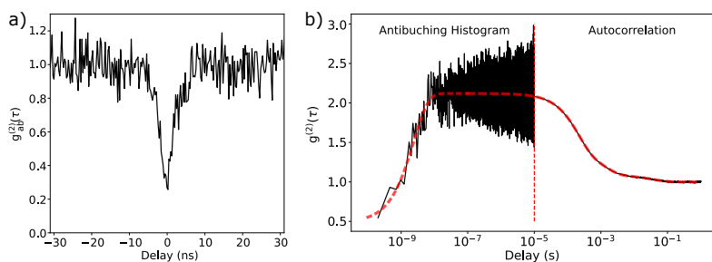
Figure 5.19.: Normalized antibunching histogram of the molecule in Figure 5.18a, measured at resonance with the 0-0 ZPL. No Rabi oscillations are present, but the characteristic time of the exponential increase to unity is shorter than for the off-resonant excitation, indicating that stimulated emission reduces the antibunching time scale. b) The full extent of the correlation function is composed for the left side by a renormalized antibunching histogram and for the right side by the calculated autocorrelation of the fluorescence signal, both recorded with an excitation intensity of around 100 W/cm 2 (see Figure 5.18d for reference).
