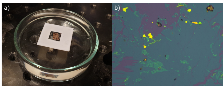
Figure 5.24.: Panel (a) shows a piece of copper foil, coated with a 13 nm thick hBN layer, floating in the middle of a hole in a Teflon slide that also floats on an etchant solution of 10% ammonium persulfate in water. Panel (b) shows hBN flakes on a substrate (most of them in yellow or green color), with areas that are encapsulated covered by a bluish film. Note that upon transfer the sheet tears and does not cover all parts of the substrate.
