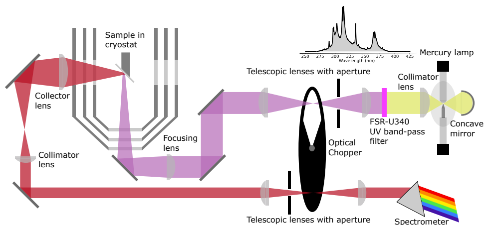
Figure 3.4.: Schematic of the phosphorescope. Starting from the top right: The collimated light from the mercury arc lamp is filtered to pass the part of the mercury spectrum as shown in Figure 3.3. The UV light is then focused on the chopper, while the beam is cleaned with an aperture. After a focusing lens, the light enters the cryostat from below, passes through the three fused silica windows, and hits the sample with a few mm beam shape. The phosphorescence is collected from the side of the cryostat by a large lens, where further on the emitted light is collimated and again focused onto the chopper and cleaned up by an aperture. Finally, the phosphorescence hits the detector of the spectrometer. Not shown here is the extensive shielding placed between the two light paths. It is important that no light leaks from the excitation path to the detection path, as it can blur weak phosphorescence signals on the spectrometer.
