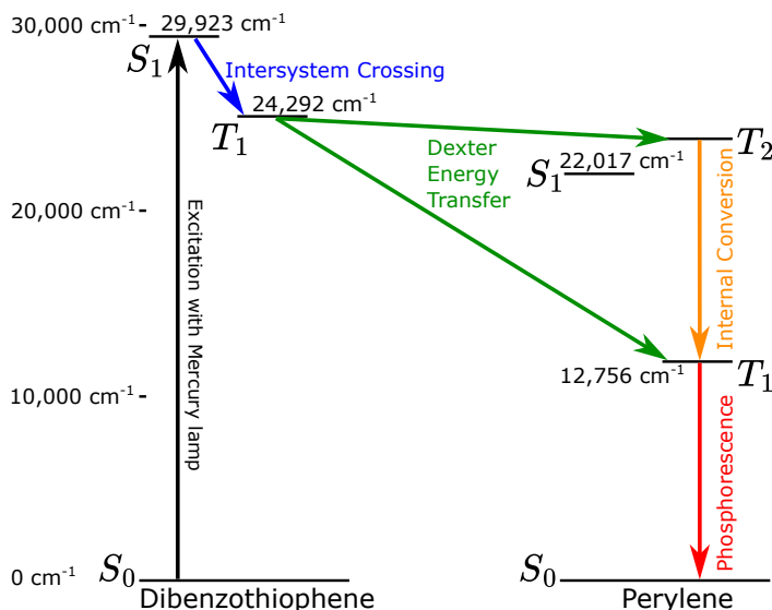
Figure 3.10.: The literature reports 13 that there might be a second triplet excited state T_2 of perylene, which is only 0.2 eV higher in energy than the singlet excited state S_1 of perylene. The energy of T_2 would therefore be slightly lower than T_1 of dibenzothiophene and therefore T_2 of perylene may participate in the energy transfer between dibenzothiophene and perylene.
