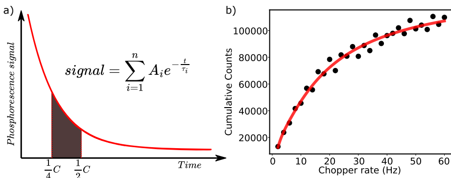
Figure 3.11.: Panel (a) shows a schematic representation of the measured integrated intensity of the exponential decay of phosphorescence in terms of the time per cycle. At an increased chopper rate the integrated area moves to the left. In steady state, the decay curve is represented by the shown formula. Panel (b) shows the integrated intensity of perylene-d12 phosphorescence measured in a single spectrum at various chopper rates. The integration time per point is 120 seconds and the line is a fit of the data to equation 3.3. The best fit is obtained by a sum of two exponential decays.
