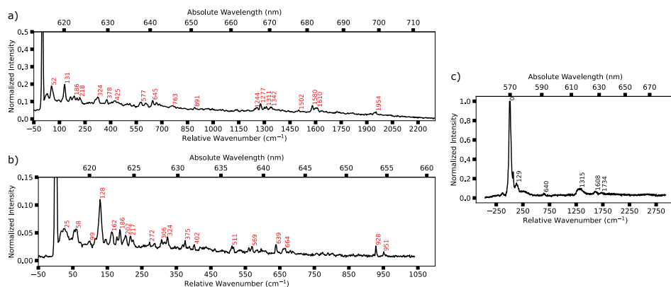
Figure 5.23.: Panel (a) shows the full emission spectrum of the C96 GQD at 2 K, excited at 570.74 nm and taken with a 600 lines/mm grating at a 0.1 mm slit size. The higher resolution spectrum, taken with a 1200 lines/mm grating and a 0.1 mm slit size, is shown in panel (b). In panel (c) an emission spectrum of the C78 GQD is shown, which was only observed at elevated temperatures. In this case the temperature is around 80 K and is responsible for the broadened linewidth. The C96 GQD molecule in (a) and (b) has a 0-0 ZPL around 615.8 nm and the C78 GQD molecule in (c) has a 0-0 ZPL around 569.7 nm.
