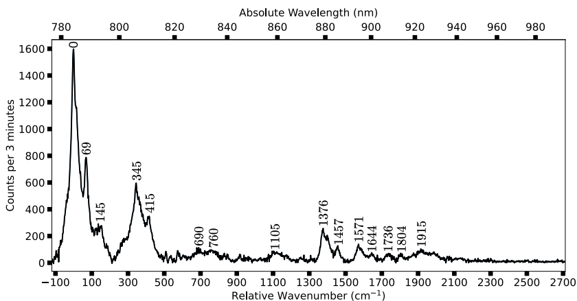
Figure 3.9.: Phosphorescence spectrum of perylene-d12 at a chopper rate of 18 Hz, imposing a delay of 15.6 ms between excitation and detection cycles. The integration time is 45 minutes in total, recorded in two sections, where single spectra are taken at a 3 minute integration time and subsequently merged. The individual spectra are used to remove cosmic rays by substitution. The vibrational fingerprint closely resembles that of the fluorescence spectrum in Figure 3 in Chapter 2, but the lines are much broader due to the high concentration of perylene-d12 and possible mixture of multiple spectroscopic sites (see section 3.3.3).
