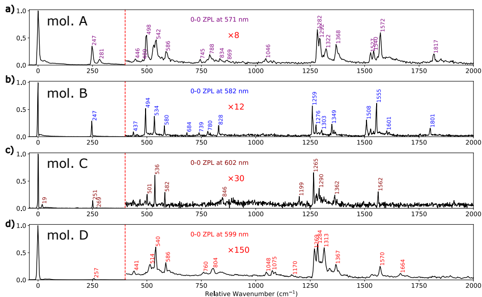
Figure 5.11.: Comparison of fluorescence emission spectra of single terrylene molecules at various positions in the inhomogeneous broadening. The spectrum in panel (a) is from a molecule with a 0-0 ZPL at 571 nm, taken on annealed hBN from NIMS. Panel (b) shows the detailed spectrum of the molecule in Figure 5.9a (blue curve), with a 0-0 ZPL at 582 nm and taken on HQ Graphene hBN (not annealed). Panel (c) shows a red-shifted molecule (602 nm) taken on HQ Graphene hBN that was annealed. Another red-shifted molecule at 599 nm is shown in panel (d), taken on annealed NIMS hBN. Note that the red-shifted molecules have weaker Franck-Condon factors, where in the extreme case of molecule D, the part of the spectrum after 400\text{ cm}^{-1} is magnified by 150x for comparison. Moreover, the phonon sidebands are weaker for the red-shifted molecules. In the case of (d), the Debye-Waller factor ( =I_{ZPL}/(I_{ZPL} + I_{PSB}) ) is more than 0.9. The spectra in (a) and (d) were taken with a slightly lower resolution of 600 lines/mm at a 0.1 mm slit size of the spectrometer in order to capture the whole spectrum at once. The spectra in (b) and (c) were taken with the higher resolution grating of 1200 lines/mm and 0.1 mm slit size and are therefore stitched by two individual recordings.
