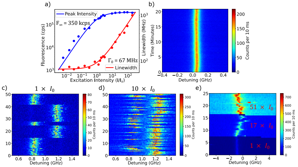
Figure 4.3.: Spectral properties of single terrylene molecules. Panel (a) shows the linewidth and fluorescence rate covered over four orders of magnitude in laser intensity for a molecule in the red site, shown here along with fits of the saturation intensity I_s . The estimated saturation intensity is in the order of 2 W/cm 2 . The red data points are the measured linewidths, which are fitted to the broadening equation \Gamma(I) = \Gamma_0 \sqrt{1 + I/I_s} . The blue data points are the measured fluorescence rates as a function of laser intensity, fitted to F(I) = F_\infty(I/I_s)/(1 + I/I_s) . Panel (b) shows another molecule in the red site that was followed in real time for more than 20 minutes with an integration time of 10 ms per point. Panel (c) and (d) show a molecule in the blue site that couples to a two-level system (TLS), that induces spectral jumps in the series of excitation spectra. Typical for TLSs, the jump rate scales with the excitation intensity. Panel (e) shows a molecule in the blue site that undergoes spectral diffusion upon increasing excitation intensities.
