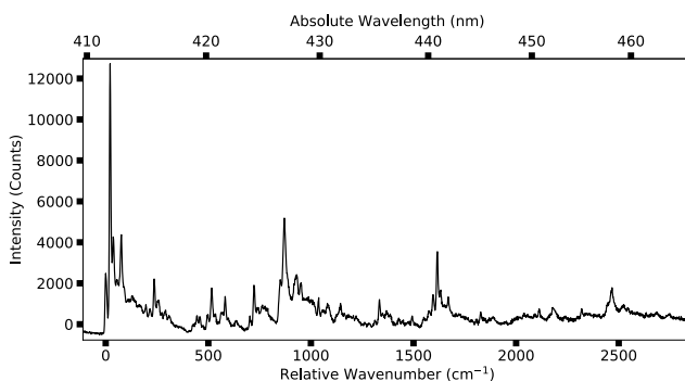
Figure 3.5.: Delayed emission spectrum of dibenzothiophene crystals doped with perylene-d12. The spectrum is recorded at 2 K, where the excited triplet remains trapped on the host molecule. The integration time of the spectrum is 6 minutes, taken with a 0.1 mm slit size and 1200 lines/mm grating. The spectrum is recorded in the second order of the grating to obtain a higher resolution. The first peak in the spectrum was chosen as the origin of the spectrum, with the relative energy of the vibrational peaks indicated in wavenumbers ( \text{cm}^{-1} ).
