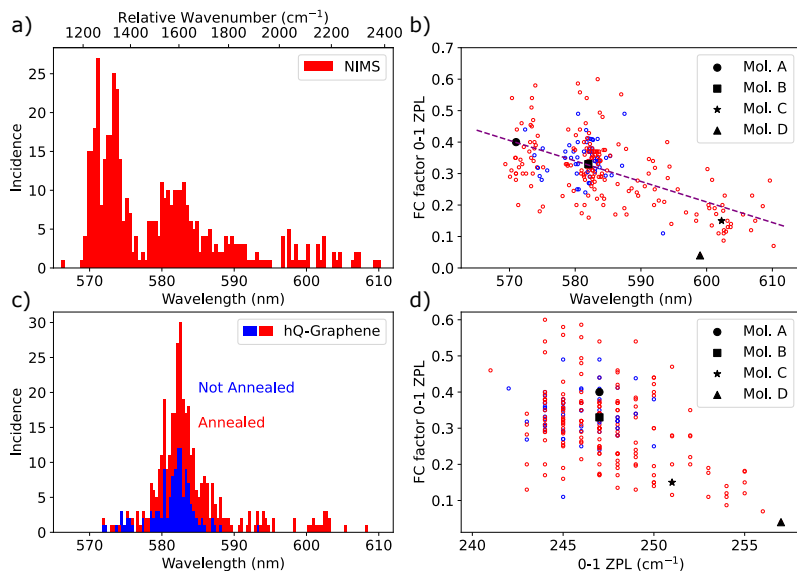
Figure 5.10.: Panel (a) displays the histogram of wavelengths where we found the purely-electronic transition of single terrylene molecules on hBN flakes from NIMS. All data was recorded with a fixed 532 nm excitation laser and for reference the relative difference in energy between this laser and the 0-0 ZPL of the molecules is shown on the top axis in wavenumbers. Note that some structure is present in the histogram, which might arise from absorption peaks that reflect the vibrational spectra in Figure 5.11 of terrylene. Hence, some molecules may not appear in the histogram, because there are no absorption lines present at 532 nm. This suggests that there might be a continuous distribution, spanning a large range of more than 40 nm. All data of 452 individual molecules is obtained from annealed hBN. Panel (b) shows for 237 molecules (58 molecules for non-annealed hBN in blue color), both from hBN from NIMS and HQ Graphene, the relation between the relative intensity of the main vibration (0-1 ZPL) versus the position of the 0-0 ZPL. On average, the more red-shifted molecules have a weaker vibronic coupling (Pearson's correlation coefficient r = -0.56 ). In panel (c) a similar distribution is shown as for (a), but for hBN from the supplier HQ Graphene and taken from both annealed (red data) and non-annealed (blue) hBN. The total number of molecules in the histogram amounts to 373 (123 for non-annealed and 250 for annealed hBN). Panel (d) shows the relation between the energy of the 0-1 ZPL and the relative intensity of the 0-1 ZPL compared to the 0-0 ZPL. Overall, a decrease in the Franck-Condon (FC) factor of the 0-1 ZPL is measured when the energy of the 0-1 ZPL is higher. The symbols displayed in panel (b) and panel (d) refer to the molecules that are plotted in Figure 5.11.
