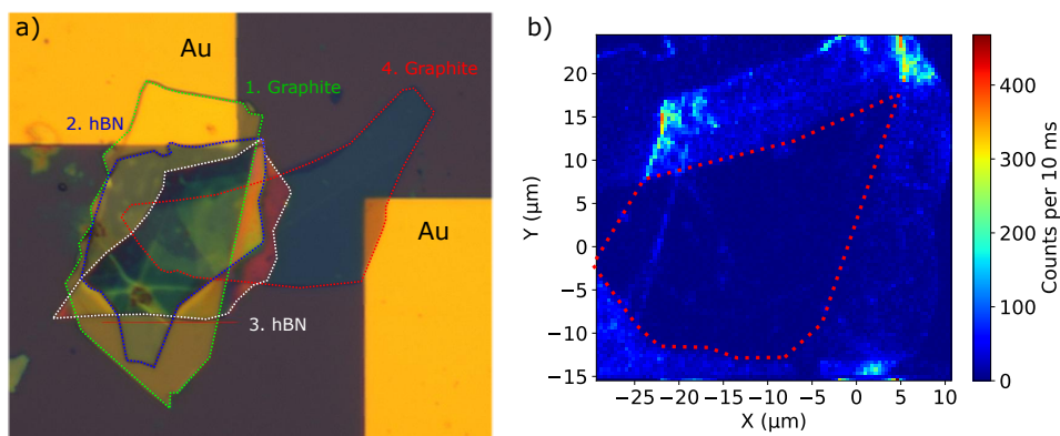
Figure 5.29.: Panel (a) shows a heterostructure with a thinner top graphite layer (see better contrast of overlap on the right electrode). Panel (b) shows the middle area of the heterostructure where all layers overlap. Some fluorescence signal is visible in the overlap region, bordered with the red dashed line.
