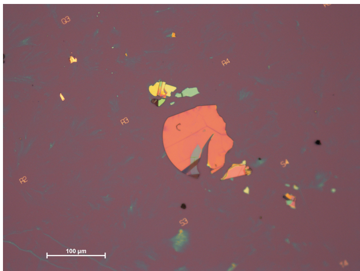
Figure 5.2.: . Microscope image of a collection of hBN flakes that are obtained by exfoliation. The sizes of the flakes vary from sub- \mu\text{m} to large flakes of up to a few 100\ \mu\text{m} . The color of the flakes gives a rough indication of the thickness, as it arises from interference of light reflected from the interfaces. 27 Typically, the bluish flakes are the thinnest, while reddish flakes are the thickest. The blue-green-yellowish clouds in the background are polymer residues from the scotch tape.
