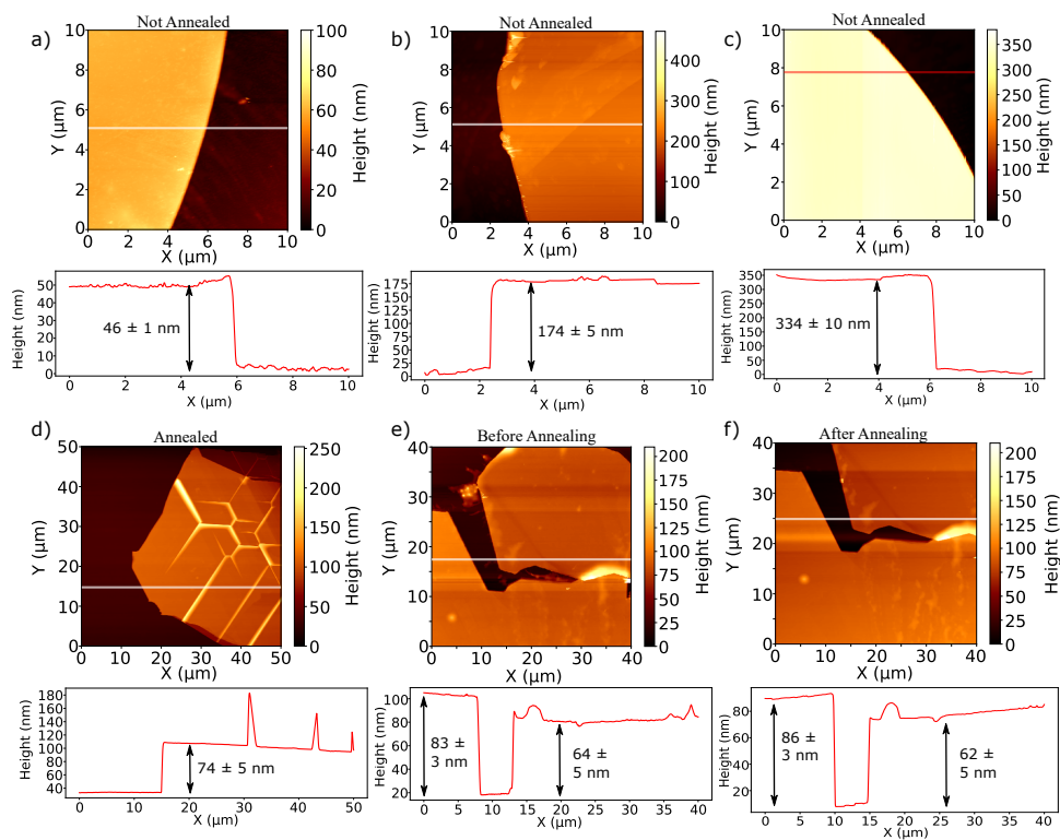
Figure 5.4.: a,b,c) AFM scans of a small part ( 10 \times 10 \mu\text{m}^2 ) of non-annealed exfoliated hBN flakes on a Si/SiO 2 substrate with below each 2D map the corresponding height profile, recorded along the white line (red for (c)). The flake in (d) is annealed at 500 °C for 12 hours. The AFM images in (e) and (f) show the same flake, respectively before and after annealing at 500 °C for 12 hours.
