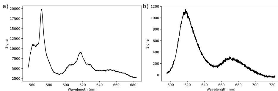
Figure 5.22.: Fluorescence emission spectra of ensembles of respectively the C78 GQD in panel (a) and the C96 GQD in panel (b). Both spectra were taken at room temperature with a 532 nm excitation laser. The spectrum in (a) peaks around 571 nm and the spectrum in (b) has a peak around 618 nm.
