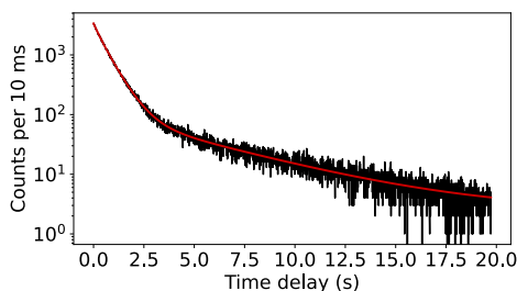
Figure 3.6.: Phosphorescence decay curve of dibenzothiophene crystals at 2 K. The integration time is 10 ms per point, measured in the spectral region determined by a band pass filter between 440-460 nm. The red curve is a fit by a sum of three exponential decays.
