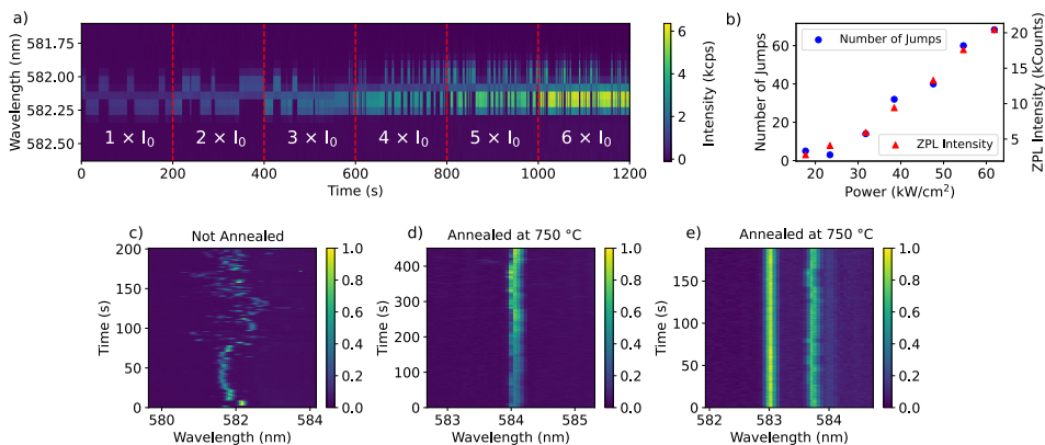
Figure 5.13.: A 0-0 zero-phonon line (ZPL) of a terrylene molecule in the main site followed for 20 minutes on an hBN flake that was annealed at 750 °C for 12 hours, excited by a vibronic transition with 532 nm light. The excitation intensity is raised after each frame of 200 s. The associated power densities, relative to the initial intensity I_0 , are shown in (b), together with the number of spectral jumps that are observed in the 200 s time window and the integrated intensity of the 0-0 ZPL for a period of 1 s. Without annealing, the spectral time trace typically exhibits complex spectral diffusion as shown for example in (c). In this case, the molecule initially wanders around a relatively narrow spectral region, but extends over a much wider region from about 70 s. After annealing, the amplitude of spectral diffusion is typically strongly reduced, as in (d), even though the laser power is doubled at each 100 s interval. Some molecules do not show any spectral diffusion on the scale resolved by the spectrometer, as is the case for the leftmost molecule in (e). The spectra in (c) are measured on a different sample than the spectra in (d) and (e).
