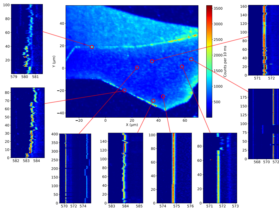
Figure 5.14.: Shown in the middle is a fluorescence image of an annealed (750 °C for 12 hours) hBN flake (NIMS, Japan). The red circles with connected lines correspond to the molecule(s) in the plotted series of spectra, with focus on the 0-0 ZPL. The two spectra on the left correspond to molecules located close to an edge, while the remaining spectra are recorded on extended terraces. The horizontal axes of the spectra correspond to the wavelength and the vertical axes correspond to the spectrum number, where each spectrum was integrated for 1 s with a 1200 lines/mm grating at a 96 μm slit size.
