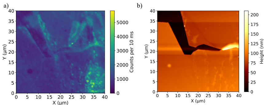
Figure 5.12.: (a) Fluorescence image and (b) AFM image corresponding to same area of a hBN flake that was annealed at 500 °C for 12 hours. The region in (a) for 25 < X < 30 \mu\text{m} and 23 < Y < 35 \mu\text{m} appears to have changed with respect to the same region in b), perhaps due to a folding of a part of the flake by the AFM tip.
