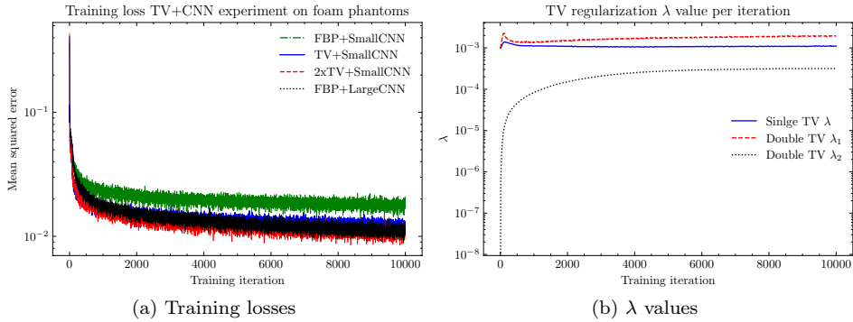
Figure 3.19: (a) Mean squared error loss during training. (b) TV regularization \lambda values during training.
