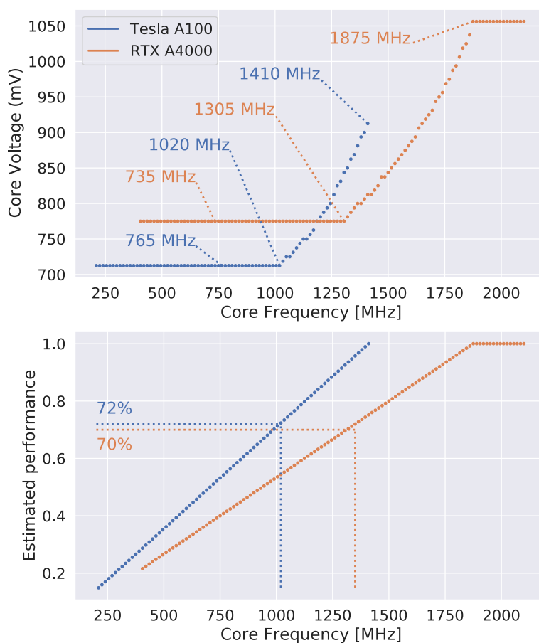
Figure 6.8: Top: GPU core frequency versus voltage curves for Tesla A100 and RTX A4000. The base clock frequency, the ridge point and peak frequency for each GPU are highlighted with a dashed line and label. Bottom: estimated performance under the assumption that GPU performance scales linearly with the clock frequency up to the point where throttling (if any) occurs. Estimated performance is normalized according to the performance for the highest possible clock frequency.
