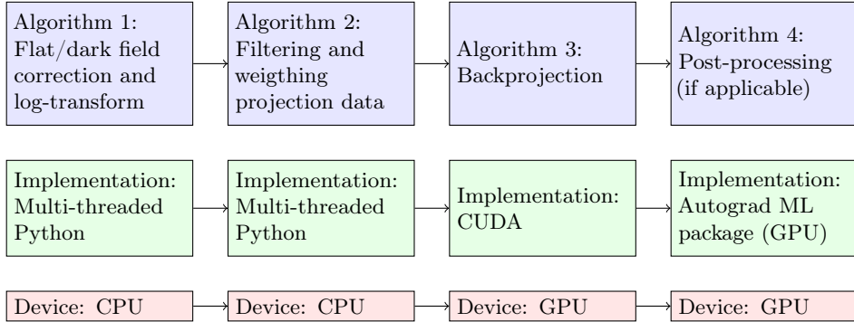
Figure 1.3: A schematic illustrating different implementation levels of an example CT imaging pipeline using FDK reconstruction.
