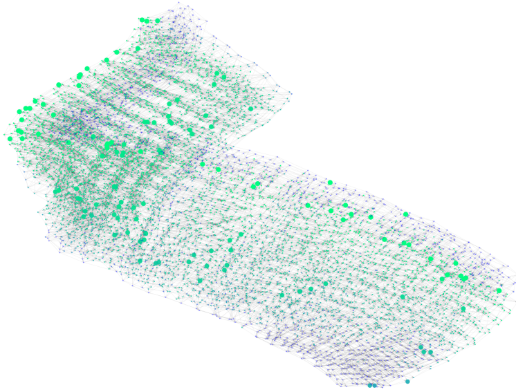
Figure 1.11: Fitness flow graph of point-in-polygon kernel search space of the Nvidia Titan RTX. Each node is a point in the search space. There is a directed edge between neighbouring points from higher to lower kernel runtime. Points are coloured within a fitness range of +25% with respect to the global minimal fitness (global minimum in green), i.e., each point is coloured by its fraction of optimal fitness, and points with a fraction below 0.75 are given the same colour. Local minima are represented as larger nodes.
