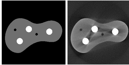
Figure 3.11: (Left): Barbpapa phantom consisting of PMMA filled with aluminium cylinders. (Right): FBP reconstructions of simulated spectral projections (with added Gaussian noise).
