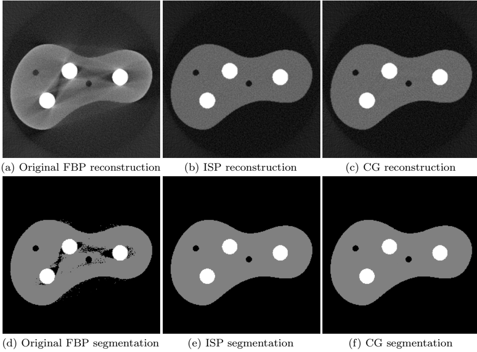
Figure 3.12: (Top): Barabapapa phantom reconstructed with the Filtered BackProjection (FBP) algorithm for ISP and a combined gradient-based (CG) approach. (Bottom): Material segmentations of corrected reconstructions.
