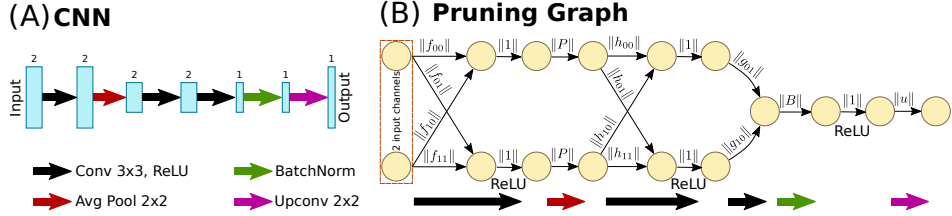
Figure 4.1: (A) Example CNN architecture with the number of channels indicated above each layer. (B) Associated pruning graph. Every channel is a node, and every operator is an edge connecting input and output nodes. The edge weights are the corresponding operator norms.
