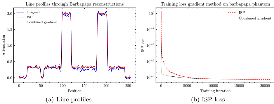
Figure 3.13: (a) Three line profiles through the original, ISP corrected, and combined gradient corrected Barabapapa reconstructions. (b) Optimization losses per \varphi evaluation.
