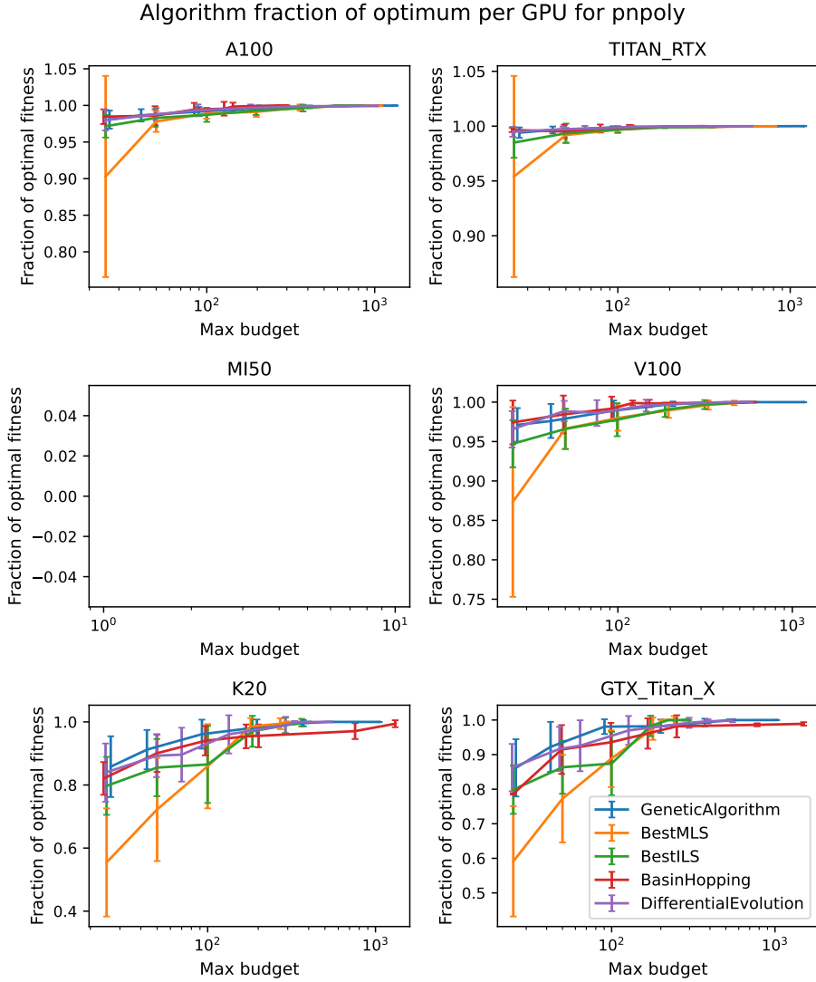
Figure A14: Point-in-polygon : Fraction of optimal runtime per GPU for GA, BestMLS, BestILS, basin hopping, and differential evolution over 50 runs. Each point is the mean fraction of optimal runtime found ( y -axis) for mean budget used (logarithmic x -axis), with error bars indicating the standard deviation in fraction of optimum. The point-in-polygon kernel was not implemented for the MI50 GPU.
