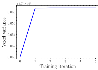
(c) Contrast measure during optimization
