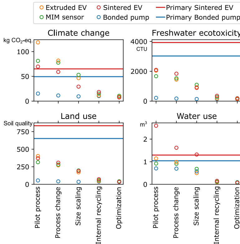
Fig. 6. Environmental impact changes due to cumulative technology developments in recycling, for four impact categories. The impacts of industrial primary magnets are shown as lines for comparison. The reference flow of each demonstrator magnet contains 1 kg NdFeB. The x-axes are shared.
