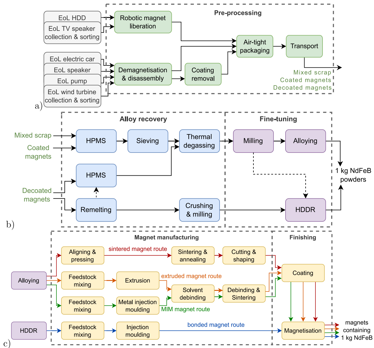
Fig. 1. Flowcharts of the studied recycling routes. The functional units (on the right) are 1 kg NdFeB powders and magnets containing 1 kg NdFeB. The system boundaries include five recycling stages, indicated by dashed outlines. Dashed arrows indicate feasible routes not fully explored in this study. HPMS: hydrogen processing of magnetic scrap; HDDR: hydrogenation-disproportionation-desorption-recombination.
