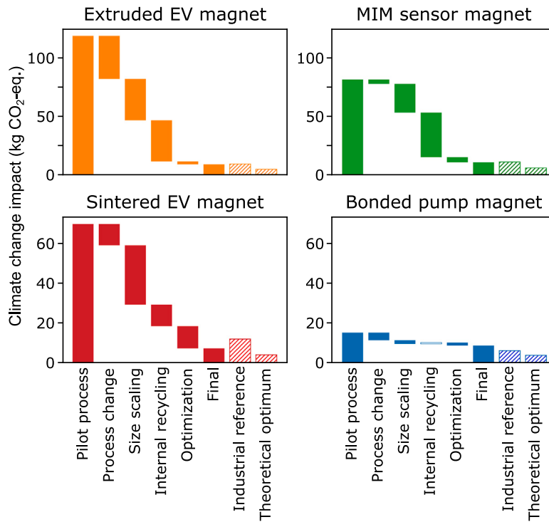
Fig. 5. Climate change impacts of 1 kg recycled demonstrator magnets. Impacts are presented for the pilot scale, after four cumulative technology improvements, and two reference configurations (dashed bars). Note that the x-axes are shared.
