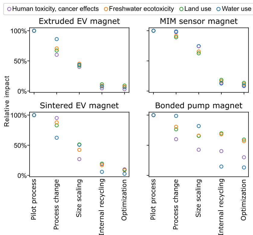
Fig. 7. Environmental impact changes due to projected technology developments for recycled demonstrator magnets, for selected impact categories. Other impact categories are provided in SI 5. The values are plotted relative to the impacts at pilot scale and the x-axes are shared.
