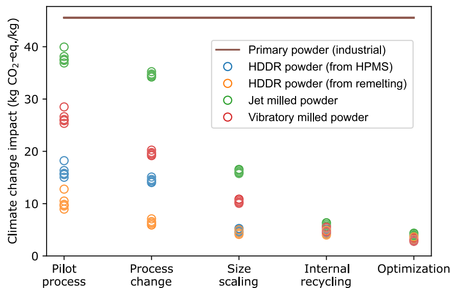
Fig. 4. Climate change impacts of NdFeB powders, from primary origin and recovered from any of six waste sources. Recovery impacts are shown for six waste sources, for the pilot scale and after four cumulative technology improvements (described in Supporting Information 1). All outputs are 1 kg of fine powders, hence milled powders have been alloyed with NdH 2 .
