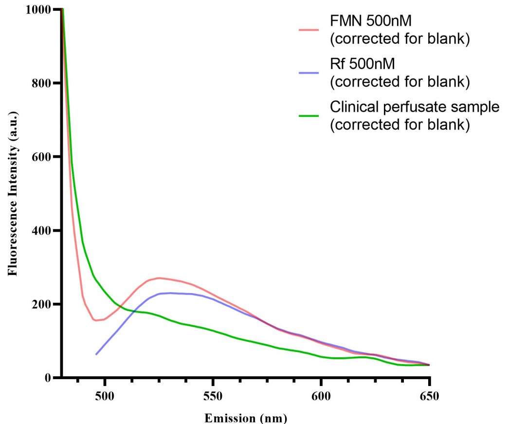
Fig 4. Comparison of fluorescence emission spectra of Flavin Mononucleotide (FMN), Riboflavin (Rf) and clinical perfusate samples. Samples (FMN 500nM, Rf 500nM and clinical perfusate sample (P3) were excited at 440nm and fluorescence emission spectra were recorded (480–650nm). Overlapping emission spectra for standards FMN (500nM) and Rf (500nM) were observed, with an emission peak at approximately 525nm. This emission peak was not observed in the fluorescence emission spectra of the clinical perfusate samples (representative sample P3 is shown), indicating that neither FMN nor Rf are present. Samples were corrected for the blank (containing UW-MPS only) and zeroed at emission 650nm.
