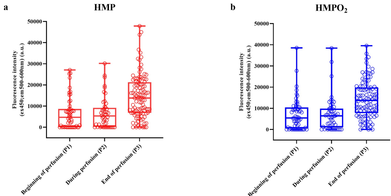
Fig 2. Change in perfusate Fluorescence Intensity ( FI_{ex450;em500-600} ) over time for HMP (A) and HMPO 2 (B). P1 perfusates were obtained 15 minutes after the start of HMP or HMPO 2 ; P2 perfusates were obtained just before leaving the donor hospital; P3 perfusates were obtained before the end of HMP or HMPO 2 . A linear mixed model was used for analysis and showed a significant increase of FI_{ex450;em500-600} over time during machine perfusion ( p < 0.0001 ). This observed increase was similar for both groups ( p = 0.83 ).
