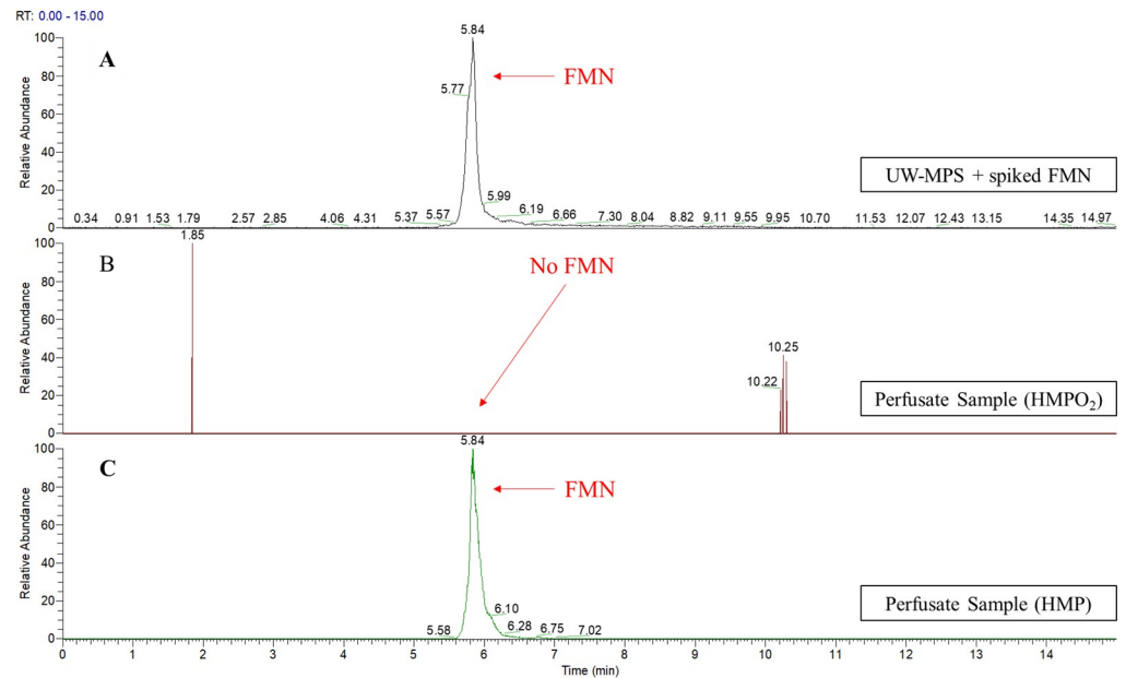
Fig 5. Representative full LC-MS chromatograms of FMN ( m/z 457.11) eluted at 5.84 minutes. (A) Chromatogram of a spiked sample with FMN concentration of 1 \mu M. (B) Representative chromatogram of the majority of perfusate samples taken at the end of perfusion (P3) where no FMN was detected. (C) Chromatogram of the only perfusate sample taken at the end of perfusion that was positive for FMN at 5.84 minutes RT.
