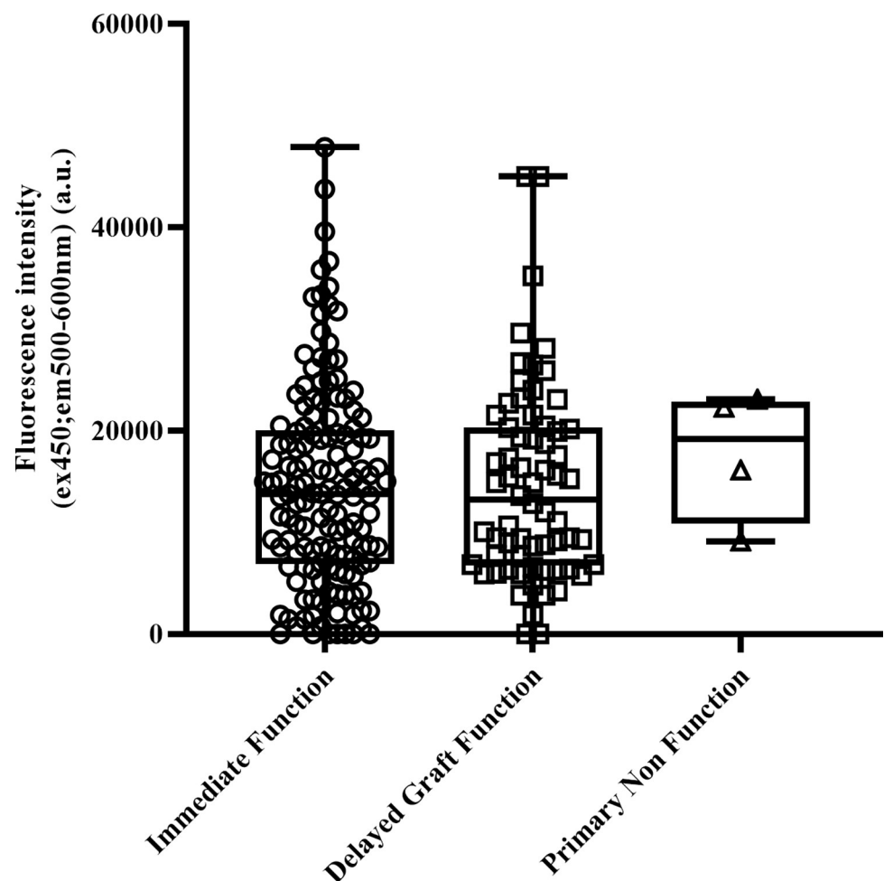
Fig 3. Fluorescence Intensity ( FI_{ex450;em500-600} ) measured in perfusate samples obtained at the end of perfusion (P3) and correlation with initial graft function of the kidney. No significant differences were observed with one-way ANOVA ( p = 0.91 ) ( FI_{ex450;em500-600} data was square root transformed to achieve normality).
