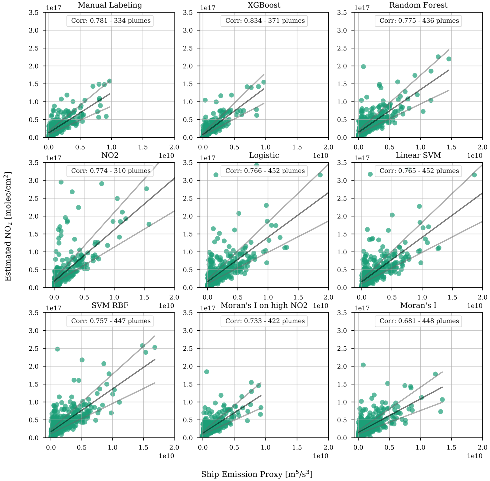
Figure 5.11: Pearson correlations between estimated (based on classification results) values of \text{NO}_2 emitted by each ship on a given day and a theoretical ship emission proxy. Black lines indicate a fitted linear trend. Grey lines show 30% deviations from the fitted linear trend.
