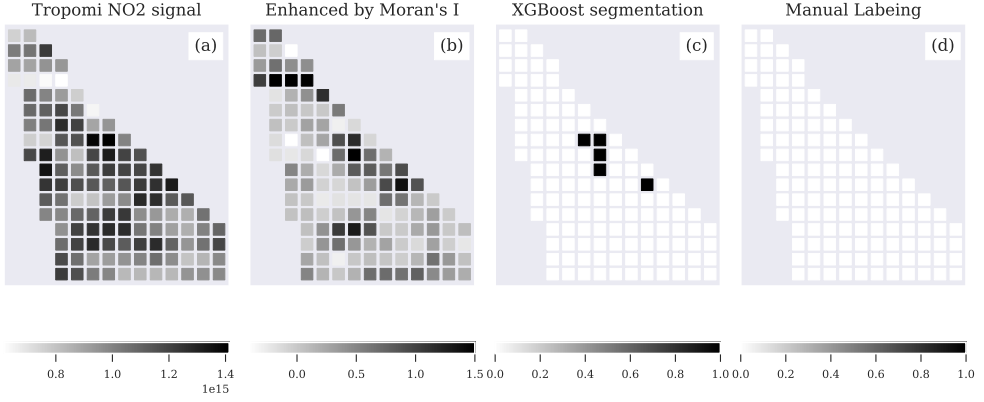
Figure 5.12: XGBoost classifier allows for the segmentation of plumes that were not recognized by the labeler. (a) TROPOMI NO 2 tropospheric vertical column density. Units: mol/m 2 . The variable was a part of the input to machine-learning models. Ship plume is difficult to distinguish by the human eye. (b) TROPOMI NO 2 image enhanced by Moran's I . The variable was a part of the input to machine-learning models. After enhancement, the ship plume can be recognized better. At the top of the ship sector can be found an example when a cluster of low value NO 2 was enhanced incorrectly. (c) Results of segmentation of XGBoost model. Black pixels indicate pixels classified by the model as a "plume". (d) Human labels. The absence of black pixels means that there were no pixels within the area labeled as a plume. For all presented images, the size of the pixel is equal to 4.2 \times 5 km 2 . Measurement date: June 24th, 2019. Ship type: Tanker. Ship length: 230 m. Average speed within the studied time scope: 14.27 kt.
