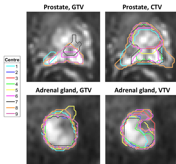
Fig. 2. Examples of delineations. Delineations made by the nine participating centres for prostate and adrenal gland, shown on b = 500 \text{ s/mm}^2 DWI images, cropped to an area of 7.7 \times 7.7 \text{ cm}^2 (prostate) and 4.9 \times 4.9 \text{ cm}^2 (adrenal gland) around the tumour. For the prostate, not all delineated contours included the shown slice, thus, only five contours are visible.
