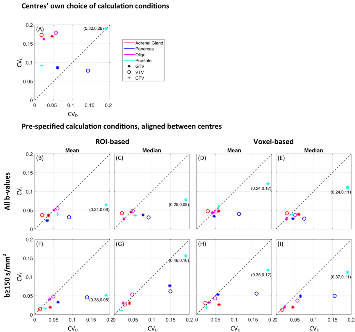
Fig. 4. ADC variation. ADC mean coefficient of variation across delineations ( CV_D ) and calculation methods ( CV_C ) from the nine MRI-linac centres, with the centres' own choice of calculation conditions (A), and with pre-specified calculation conditions (B–I). Median ADC values were used in (A). The marker colours and types represent the different clinical cases and types of ROIs. The dotted line at x = y represents the points where delineation- and calculation-related ADC variation are the same. For the prostate GTV, CV_D is outside the axis range, and therefore, the true coordinates are indicated next to the marker.
