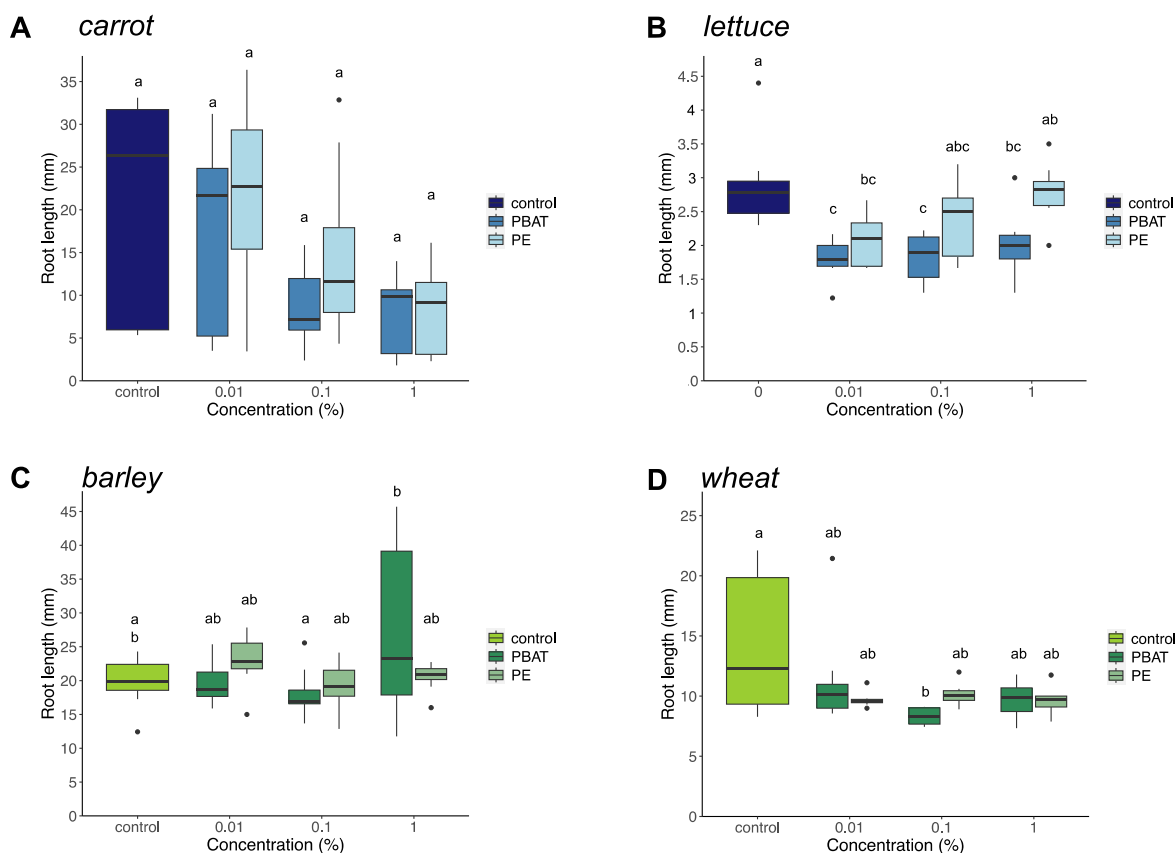
Fig. 1. The mean \pm SE root length of carrot ( Daucus carota , [A]), lettuce ( Lactuca sativa , [B]), barley ( Hordeum vulgare , [C]) and wheat ( Triticum aestivum L., [D]) buds after exposure to low, medium and high PE and starch-PBAT blend concentrations (0.01, 0.1, 1 % w/w). Lettuce, barley and wheat seeds were germinated for four days, and carrot seeds for ten days. Different letters indicate significant differences (ANOVA followed by Tukey's post-hoc test, p < 0.05 ) between treatments. Please note the high variance in the controls of carrot (A) and wheat (D).
