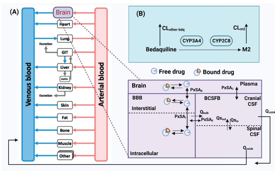
Figure 6.1. Illustration of the Bedaquiline-M2 whole-body PBPK model with CNS. The whole-body PBPK model for bedaquiline and M2 was developed in PK-Sim 19-21 . Enzymatic metabolism from bedaquiline to M2 is driven by CYP3A4 and CYP2C8. Additionally, bedaquiline is eliminated at clearance rate CL_{other-bdq} and M2 is eliminated at rate CL_{M2} . There are four routes for unbound drugs to distribute within CSF and brain – (1) from plasma into brain interstitial space, from brain interstitial into brain intracellular, and (2) from plasma into cranial CSF, then into spinal CSF, (3) from cranial CSF to intracellular space, (4) from cranial and spinal CSF into venous blood plasma. Drugs in interstitial and intracellular spaces can bind to the compartment lipid and protein content. The drug goes through mass transfer driven by CSF flow within cranial and spinal sub-compartments of CSF and also to vascular blood. BBB=blood-brain barrier, BCSFB=blood-cerebrospinal fluid barrier, CL_{other-bdq} =additional bedaquiline hepatic clearance (other than M2-relevant clearance), CL_{M2} =M2 clearance, CSF=cerebrospinal fluid, PxSA_B =permeability surface area product for BBB, PxSA_C =permeability surface area product for BCSFB, PxSA_E =permeability surface area product from brain intracellular to cranial CSF, Q_{bulk} =mass transfer flow rate from intracellular to cranial CSF, Q_{csink} =CSF flow rate from cranial CSF to peripheral venous blood, Q_{sin} =CSF flow rate from cranial CSF to spinal CSF, Q_{sout} =CSF flow rate from spinal CSF to cranial CSF, Q_{ssink} =CSF flow rate from spinal CSF to peripheral venous blood. Figure generated using Biorender.com.
