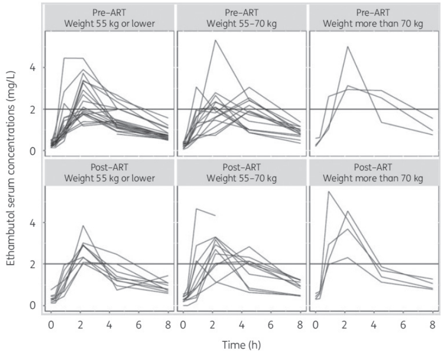
Figure 2.1 Individual ethambutol serum concentration–time curves by weight group and study visit, before and after initiation of ART. The weight group 55 kg or lower includes one patient with body weight <40 kg. The horizontal line corresponds to the proposed target range for serum ethambutol C max (2–6 mg/L).
