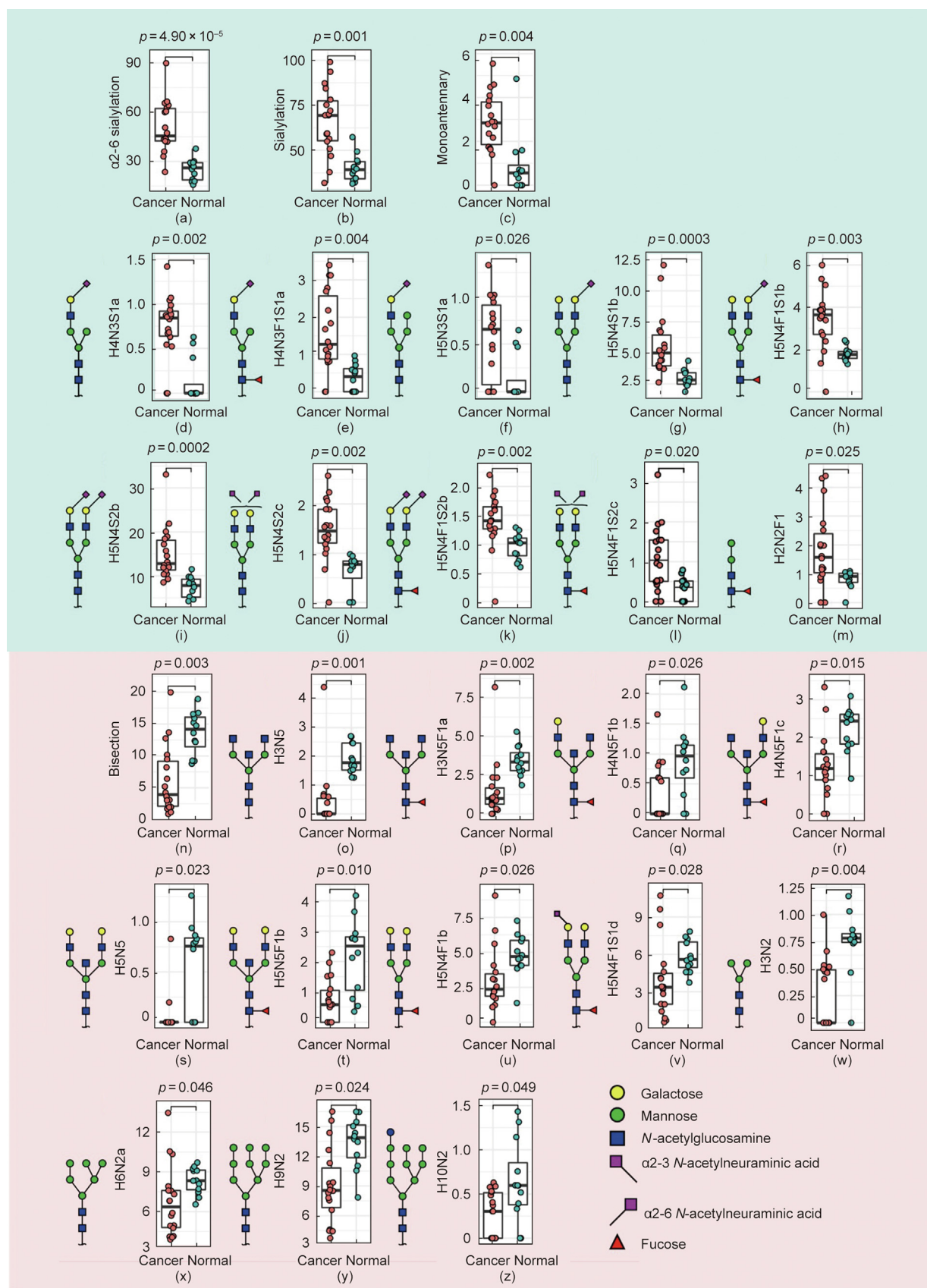
Fig. 3. Relative abundance of N -glycans and glycosylation features significantly (a–m) upregulated and (n–z) downregulated in CRC. (a–c) The N -glycosylation features (a) \alpha 2-6 sialylation, (b) sialylation, and (c) monoantennary glycans, as well as (d–m) ten individual N -glycans ((d, e) two monoantennary, (f) one hybrid, (g–l) six complex, and (m) one paucimannosidic species) were found to be significantly upregulated in CRC. In contrast, the expression of (n) bisected N -glycans and (o–z) 12 individual N -glycans were found to be higher in the normal mucosa in comparison with CRC. The Wilcoxon–Mann–Whitney non-parametric statistical test was applied to test differences between groups. Benjamini–Hochberg corrected p -values are shown above each boxplot. Y axes give relative abundance values of individual glycans and glycosylation features.
