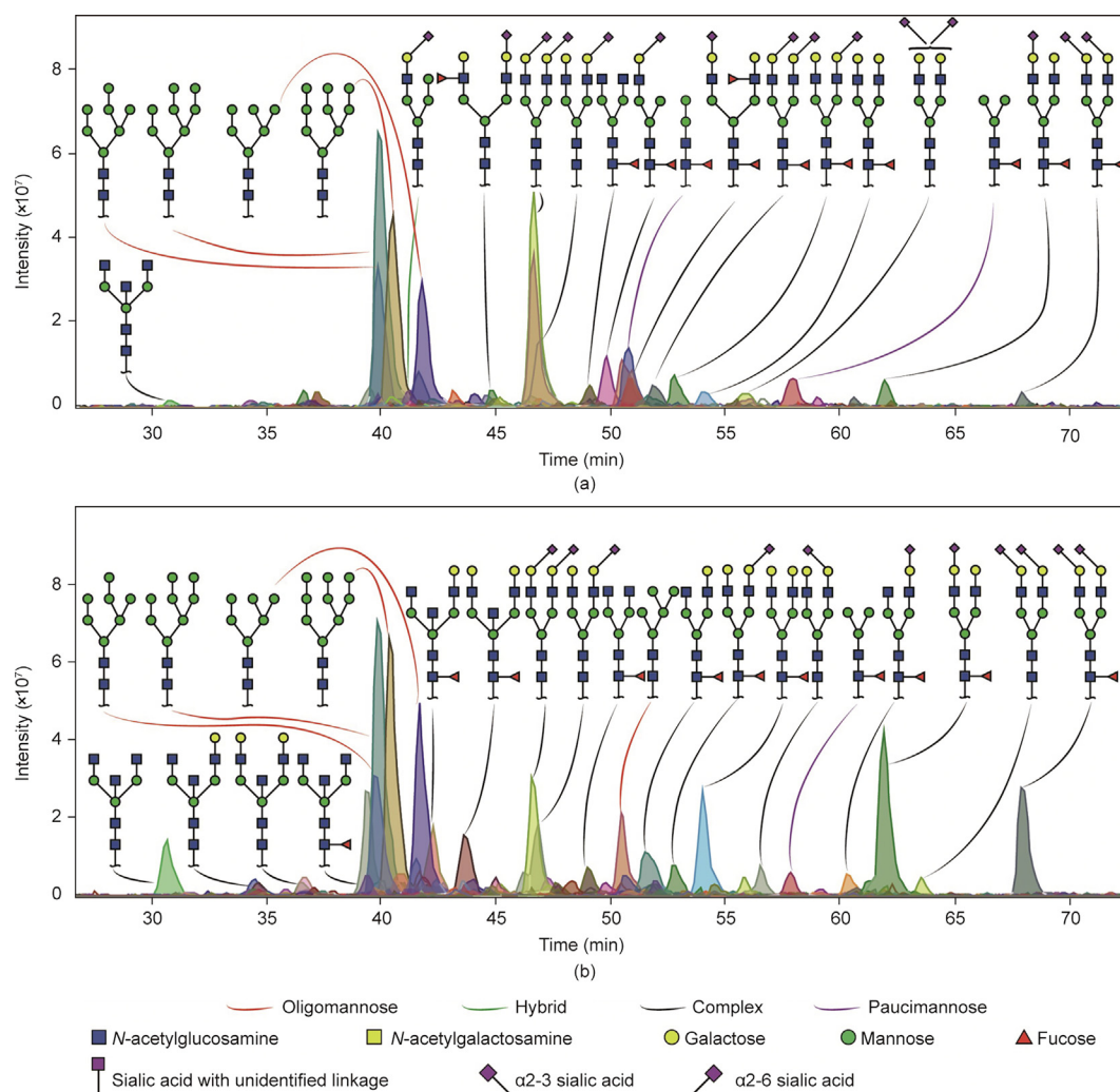
Fig. 2. Examples of N -glycan profiles of (a) adenocarcinoma and (b) normal colon mucosa from the same patient. (a) Adenocarcinoma obtained from Patient 11 was characterized by a higher expression of monoantennary N -glycans and by N -glycans carrying terminal Le A/X epitopes. In addition, more paucimannose and complex N -glycans carrying \alpha 2-6 sialic acid(s) were expressed compared with (b) normal colon mucosa from the same patient, which shows a higher expression of bisected and complex N -glycans carrying \alpha 2-3 sialic acid(s).
