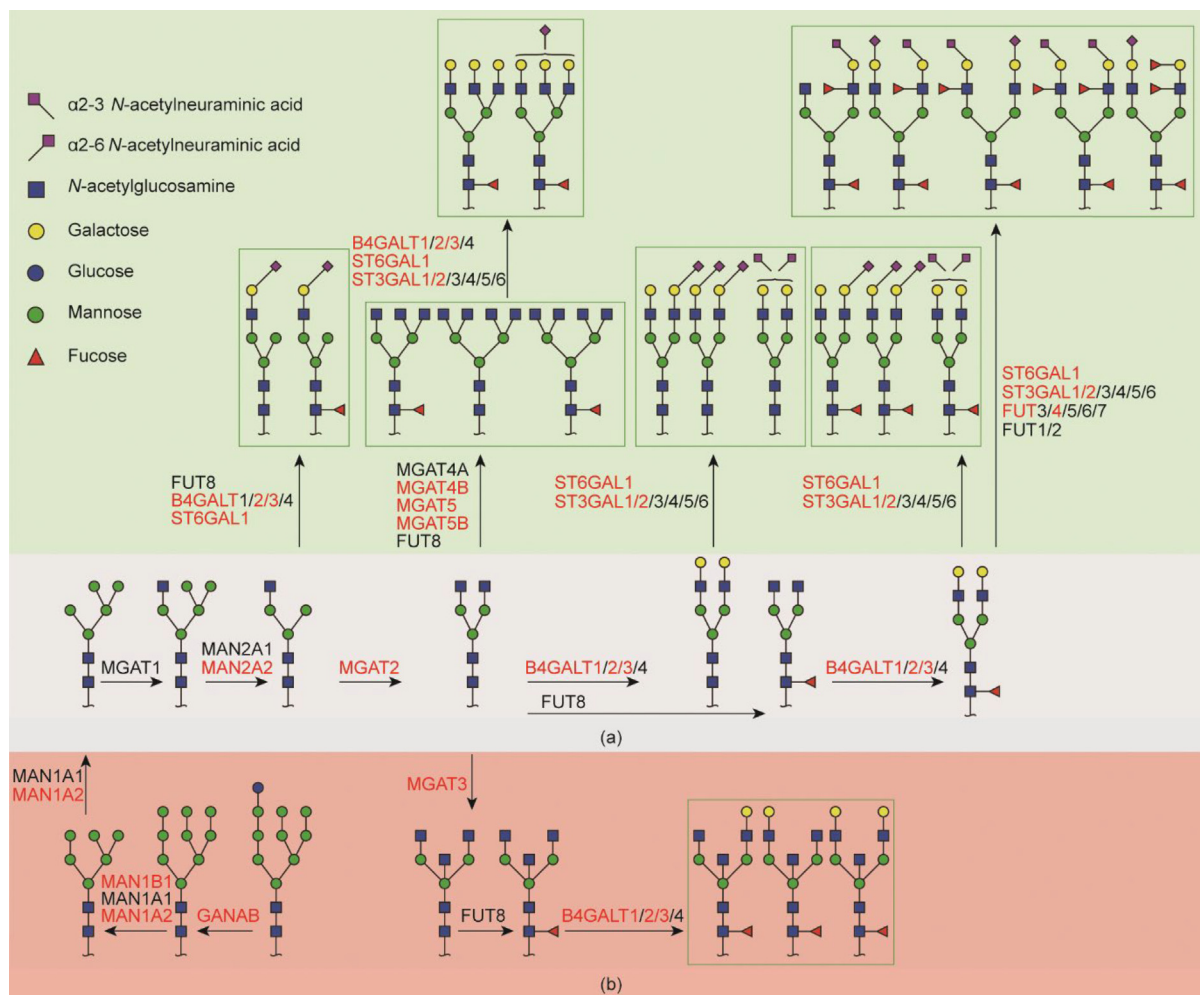
Fig. 6. Proposed biosynthetic model depicting the differences in the N-glycosylation of CRC and normal colon mucosa. High relative abundance and specific expression of N-glycans in (a) cancer and (b) normal mucosa, combined with genes encoding corresponding GTs involved in the biosynthesis of N-glycans. GT genes that are upregulated in cancer are shown in red.
