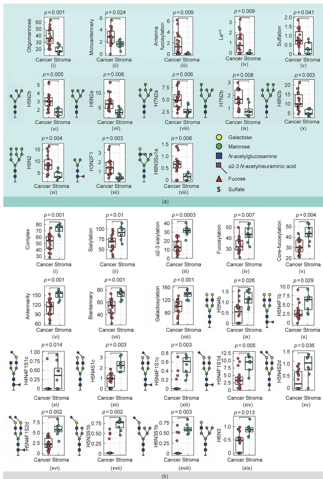
Fig. 5. Relative abundances of N-glycans and glycosylation features upregulated in CRC and in cancer stroma. N-glycosylation features indicated in (a) (blue): (i) oligomannoside, (ii) monoantennary, (iii) antenna fucosylation, (iv) Le x , (v) sulfation. In addition, eight N-glycans including (vi–xi) six oligomannosidic types, (xii) one paucimannosidic (H3N2F1), and (xiii) one hybrid-type sulfated N-glycan (H6N3Su1a) were found to be significantly upregulated in CRC. In comparison with cancer, the stroma in (b) (grey) was characterized by (i) a high expression of complex N-glycans, (ii, iii) α2-3 sialylation, (iv, v) (core-)fucosylation, (vi, vii) (bi)antennary glycans, and (viii) galactosylation; there were also (ix–xix) 11 individual N-glycans, mostly expressing α2-3 sialylation. The Wilcoxon–Mann–Whitney non-parametric statistical test was applied to test differences between groups. Benjamini–Hochberg corrected p-values are shown above each boxplot. Y axes give relative abundance values of individual glycans and glycosylation features.
