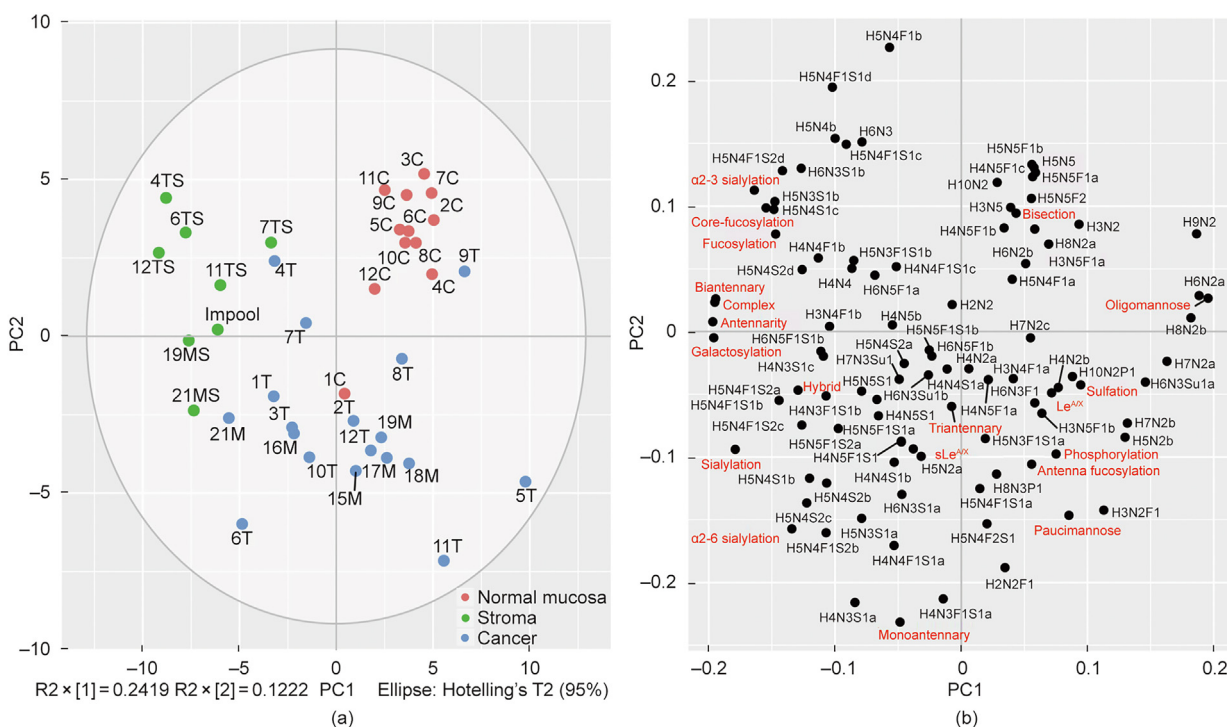
Fig. 1. Distinct glycosylation features in CRC, stroma, and normal colon mucosa. (a) The first two principal components ( R^2 \times [1] and R^2 \times [2] ) of the principal component analysis (PCA) model explain 36% of the variance. The prominent separation between CRC, stroma and normal colon mucosa is illustrated in the principal component (PC) analysis score plot of PC1 against PC2. (b) The loading plot indicates the variables driving the separation of the samples, including individual N -glycans (black) and glycosylation features (red). C: normal mucosa; T: CRC; M: CRC metastasis; S: stroma; MS: stroma of a metastatic tumor; TS: stroma from the primary tumor; R^2 \times [1] and R^2 \times [2] give the variance of the first and second principal component, respectively. More information about the glycosylation features can be found in Table S2.
