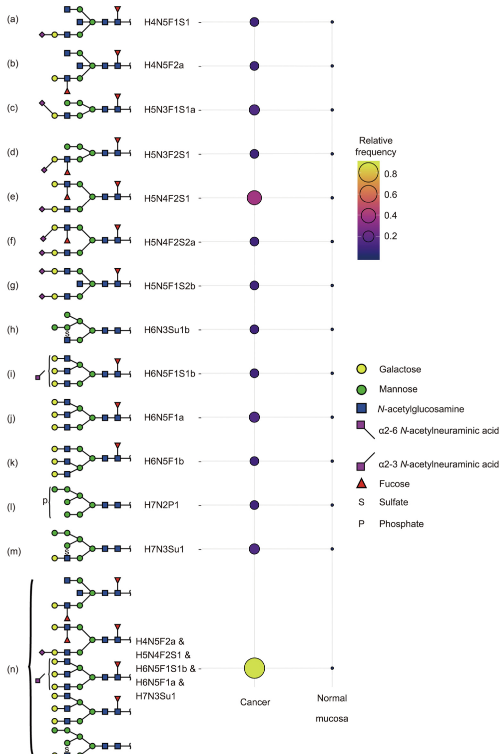
Fig. 4. Selected N -glycans with the highest sensitivity for CRC. (a–m) N -glycans were solely detected in two or more CRC samples and were absent in the normal colon mucosa. (n) At least one of the five illustrated N -glycans (either carrying sLe A/X /Le A/X epitopes or showing triantennarity) was detected in 89% of CRC samples.
