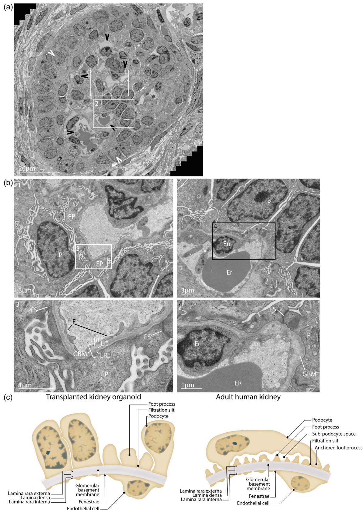
FIGURE 1 Development of the renal corpuscle of transplanted kidney organoids visualized using Transmission Electron Microscopy.
