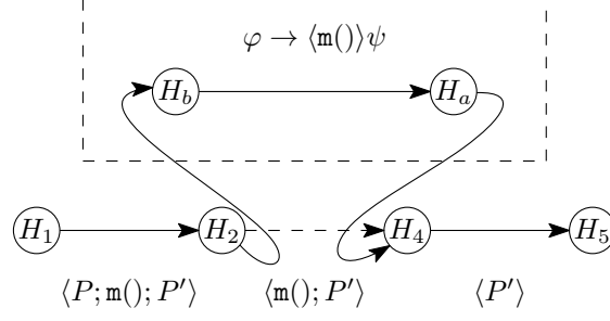
Figure 2.3: Heaps are ‘threaded’ through method calls. In heap H_1 the program fragment P is executed, resulting in heap H_2 . Either a contract for method \mathbf{m}() is employed, which relates the before heap H_b to some heap after the method call H_a ; or, the method body is unfolded by wrapping it in a method frame that resolves overshadowing of program variables. In both cases, to call the method, heap H_b is equal to H_2 and heap H_a is equal to H_4 . Then the program fragment P' that occurs after the method call is executed using the heap returned by the method.
