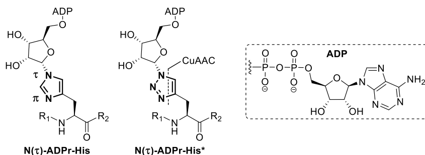
Figure 1 | Proposed structure of ADP-ribosylated histidine (N( \tau )-ADPr-His), including the \tau and \pi nomenclature for the imidazole nitrogen atoms, versus the ADP-ribosylated histidine isostere (N( \tau )-ADPr-His*) that has the imidazole functionality replaced by a triazole moiety.
