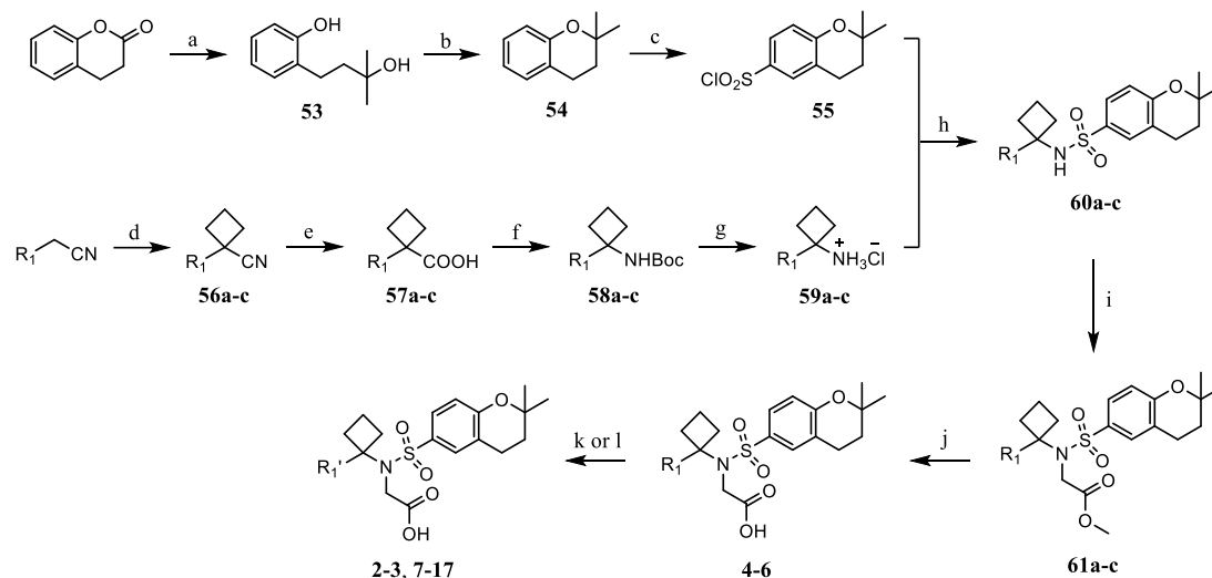
Scheme 3.1 Synthesis of glycine sulfonamides 2-17 . Reagents and conditions: a) \text{CH}_3\text{MgBr} , anhydrous THF, 0\text{ }^\circ\text{C} -rt, 84%; b) 15% aq. \text{H}_2\text{SO}_4 , toluene, reflux, 72%; c) \text{HSO}_3\text{Cl} , anhydrous DCM, 0\text{ }^\circ\text{C} -rt, 63%; d) 1,3-dibromopropane, TBABr, KOH, toluene, \text{H}_2\text{O} , reflux, 33-61%; e) KOH, ethylene glycol, reflux, 50-92%; f) DPPA, \text{Et}_3\text{N} , anhydrous t -BuOH, 30\text{ }^\circ\text{C} -reflux, 42-85%; g) 3 M aq. HCl in MeOH, rt, 93%-quant.; h) \text{Et}_3\text{N} , anhydrous DCM, rt, 46-89%; i) methyl 2-bromoacetate, BEMP, anhydrous DMF, 80\text{ }^\circ\text{C} , 90%-quant.; j) 1 M or 2 M aq. NaOH, MeOH/THF, rt, 47-quant.; k) corresponding boronic acid, \text{K}_2\text{CO}_3 , \text{Pd}(\text{dppf})\text{Cl}_2\cdot\text{CH}_2\text{Cl}_2 , 1,4-dioxane/ \text{H}_2\text{O} , 80\text{ }^\circ\text{C} , 12-75% for 2-3 , 9-17 ; l) \text{Pd}(\text{OAc})_2 , \text{K}_4\text{Fe}(\text{CN})_6\cdot 3\text{H}_2\text{O} , \text{Na}_2\text{CO}_3 , i -PrOH, \text{H}_2\text{O} , DMF, 100\text{ }^\circ\text{C} , 45% for 7 ; 30% \text{H}_2\text{O}_2 , 2 M aq. NaOH, MeOH, rt, 39% for 7 \rightarrow 8 .
