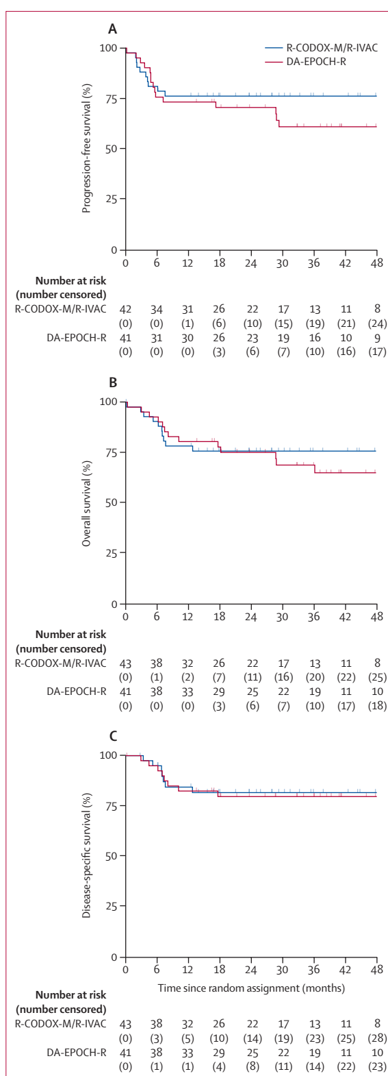
Figure 2: Kaplan-Meier survival curves
