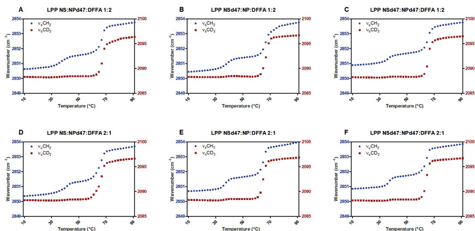
Figure S2. Thermotropic curves of the \nu_sCH_2 and \nu_sCD_2 vibrations for the CER NS:CER NP 1:2 and 2:1 ratio models with different deuterated chains. The wavenumbers of the \nu_sCH_2 and \nu_sCD_2 peak positions (left and right y-axis) are plotted in the 10-90 ^{\circ}C temperature range. Data shown as an average of 3 measurements for each composition.
