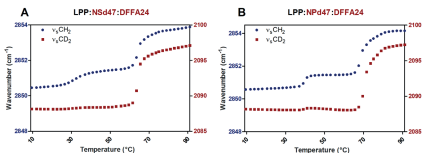
Figure S2. Thermotropic curves of the stretching vibrations for the partially deuterated systems: (A) LPP:NSd47:DFFA24 and (B) LPP:NPd47:DFFA24. The phase transitions temperatures of the lipids are plotted as a function of the \nu_s\text{CH}_2 and \nu_s\text{CD}_2 peak position, on the left and right y-axis, respectively. Both the protiated (blue circle) and deuterated (red square) lipids melted over the same temperature range, indicating that the deuterated lipids were integrated with the protiated lipids in the lipid system.
