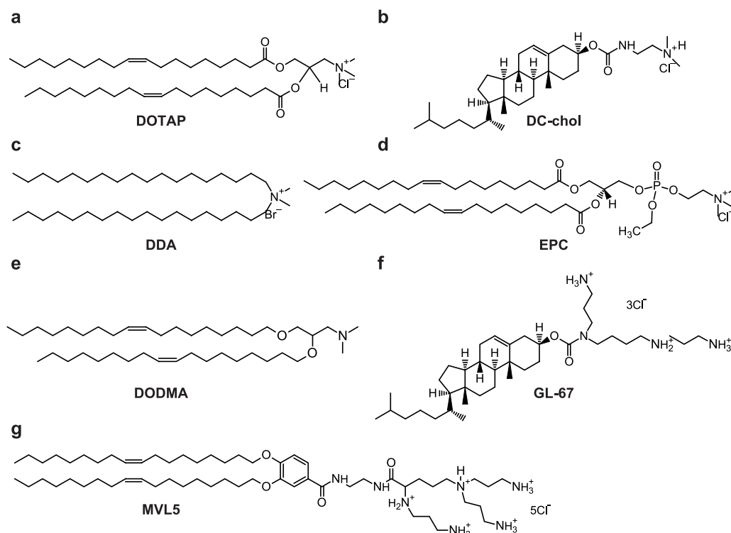
Fig. 2. Molecular structures of cationic compounds. a) DOTAP: 1,2-dioleoyl-3-trimethylammonium-propane (chloride salt), b) DC-chol: 3β-[N-(N',N'-dimethylamino)ethane]-carbamoyl]cholesterol hydrochloride, c) DDA: dimethyloctadecylammonium (bromide salt), d) EPC: 1,2-dioleoyl- sn -glycero-3-ethylphosphocholine (chloride salt), e) DODMA: 1,2-dioleoyloxy-3-dimethylaminopropane, f) GL-67: N + -cholesteryl-spermine hydrochloride, and g) MVL5: N1-[2-((1S)-1-[(3-aminopropyl)amino]-4-[di(3-amino-propyl)amino]butylcarboxamido)ethyl]-3,4-di[oleyl]oxy-benzamide.
