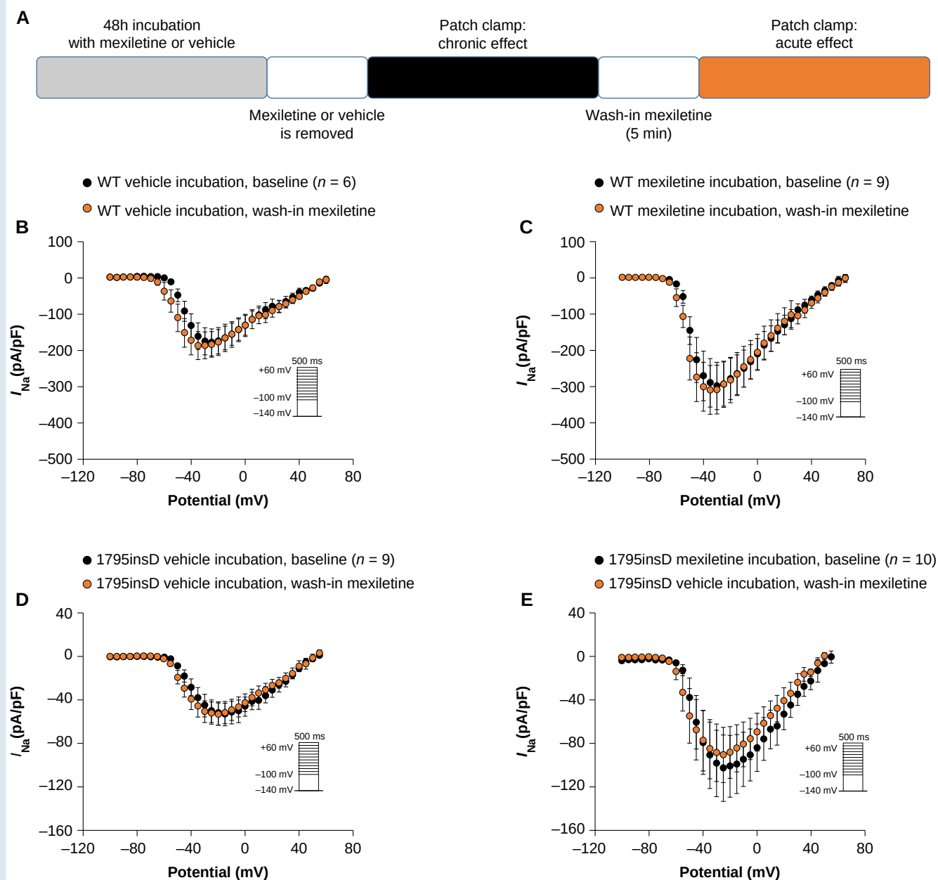
Figure 2 Acute mexiletine treatment does not affect peak I_{Na} in HEK293A cells transfected with SCN5A-WT or SCN5A-1795insD previously incubated with either vehicle or mexiletine. (A) Schematic representation of the performed experiments. (B–E) Average peak I_{Na} I - V relationships before (baseline) and after 5 min wash-in of 10 \mu M mexiletine in HEK293A cells transfected with SCN5A-WT (B, C) or SCN5A-1795insD (D, E), following 48 h incubation with either vehicle or mexiletine. WT, wild-type.
