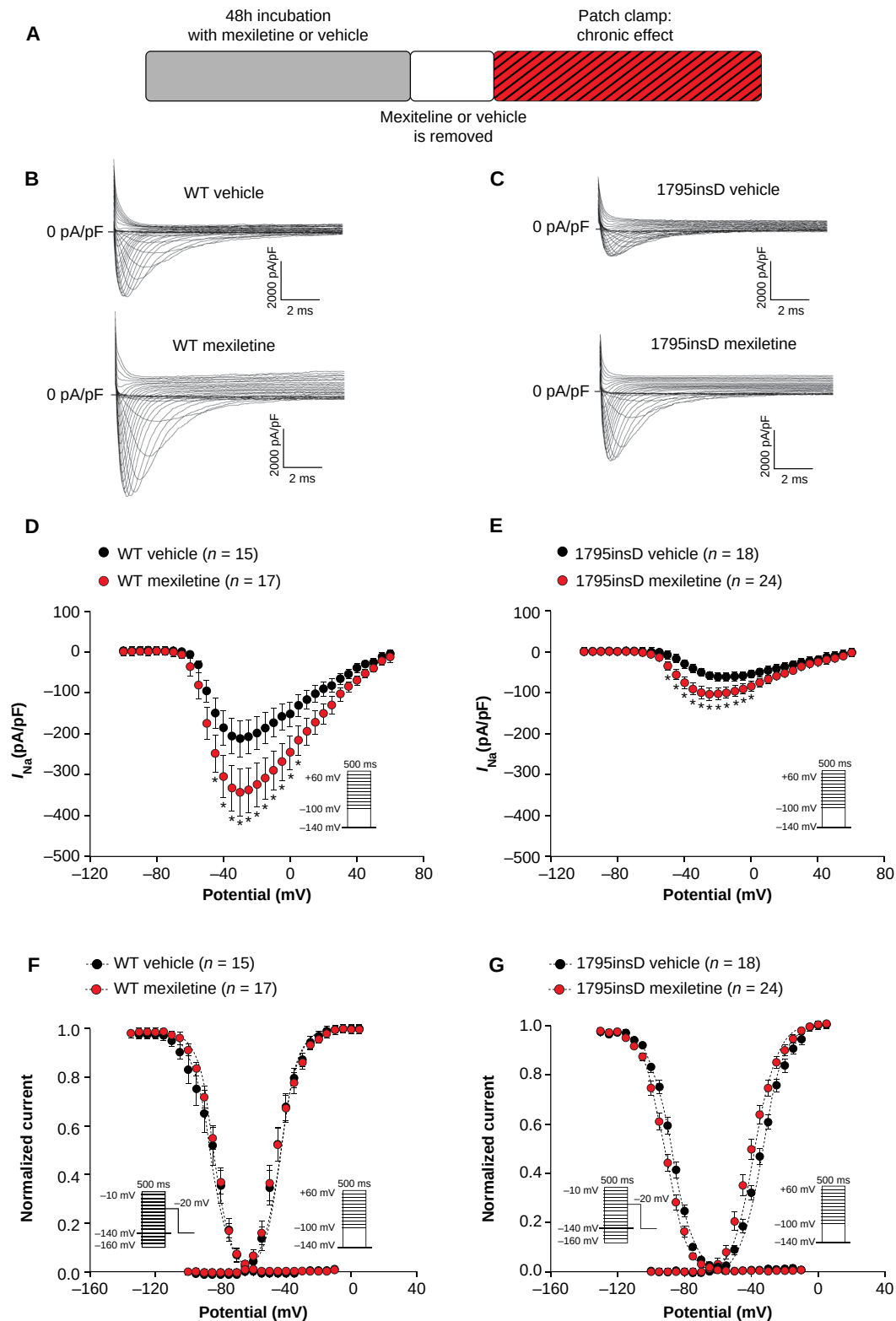
Figure 1 Forty-eight hour incubation with 10 \mu M mexiletine increases peak I_{Na} in HEK293A cells transfected with SCN5A-WT or SCN5A-1795insD. (A) Schematic representation of the performed experiments. (B, C) Representative I_{Na} traces recorded in HEK293A cells transfected with either SCN5A-WT (B) or SCN5A-1795insD (C) following 48 h incubation with vehicle or mexiletine (10 \mu M). (D–G) Average peak I_{Na} current–voltage ( I – V ) relationships (D, E) and voltage dependence of activation and inactivation (F, G) in HEK293A cells transfected with SCN5A-WT or SCN5A-1795insD following 48 h incubation with vehicle or mexiletine (10 \mu M). Insets: voltage protocols; * P < 0.05 , two-way RM ANOVA followed by Holm–Sidak test for post hoc analysis. WT, wild-type.
