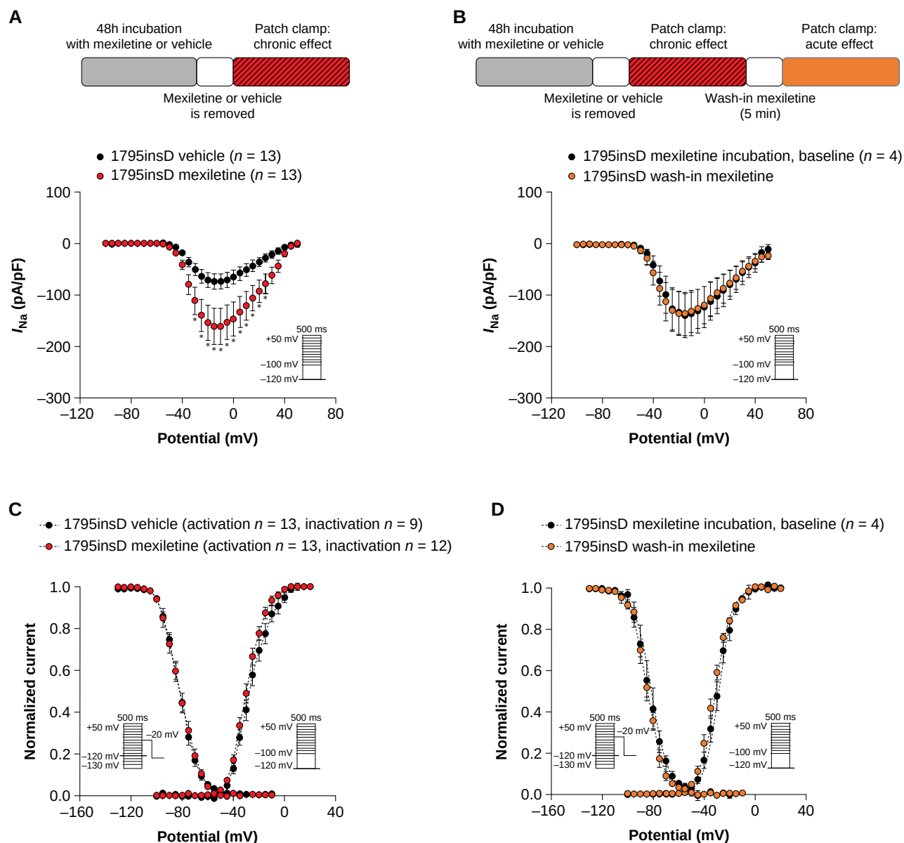
Figure 6 Forty-eight hour incubation with 10 \mu M mexiletine increases peak I_{Na} in SCN5A-1795insD hiPSC-CMs while acute mexiletine has no effect. (A, B) Schematic representations of the performed experiments (see panels) and average peak I_{Na} I - V relationships for SCN5A-1795insD hiPSC-CMs after 48 h incubation with vehicle or mexiletine (10 \mu M) followed by removal of the drug (A) and after 5 min of re-administration (wash-in) of mexiletine (10 \mu M) (B). (C, D) Voltage dependence of (in)activation measured in SCN5A-1795insD hiPSC-CMs after 48 h incubation with vehicle or mexiletine (10 \mu M) followed by removal of the drug (C) and after 5 min re-administration (wash-in) of mexiletine (D). Insets: voltage protocols; * P < 0.05 , two-way RM ANOVA followed by Holm-Sidak test for post hoc analysis.
