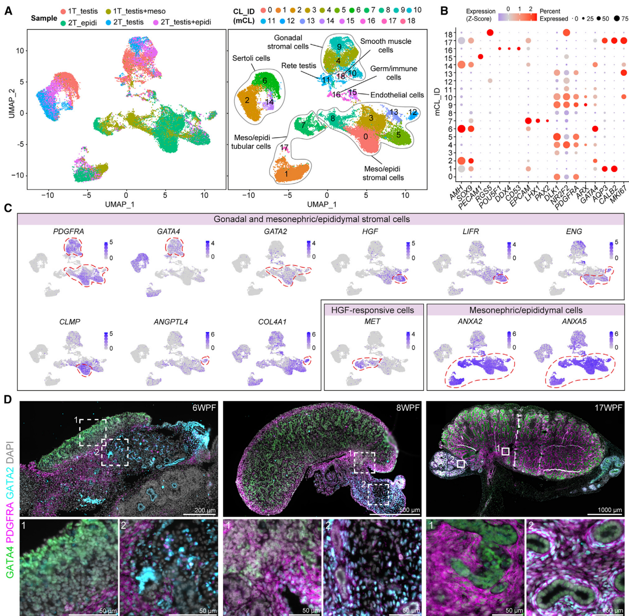
Figure 2. Molecular characterization of cell types in the human fetal male gonad and reproductive tract
