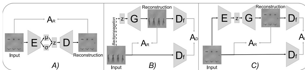
Fig. 6. Generative unsupervised anomaly detection architectures: (A) VAE with Reconstruction Error, (B) AnoGAN (Schlegl et al., 2017), (C) f-AnoGAN (Schlegl et al., 2019).
