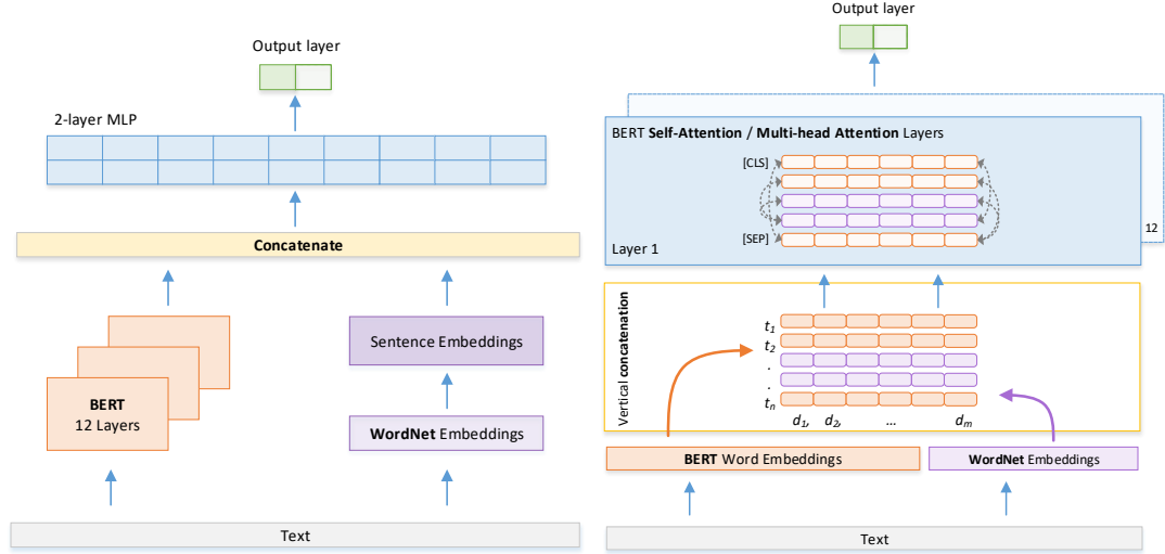
Figure 1: The model with external learning of Figure 2: The model of internal inclusion in-embeddings combination using a 2-layer MLP tegrating WordNet embeddings into BERT, top classifier. based on the approach of VGCN-BERT (Lu et al., 2020).
