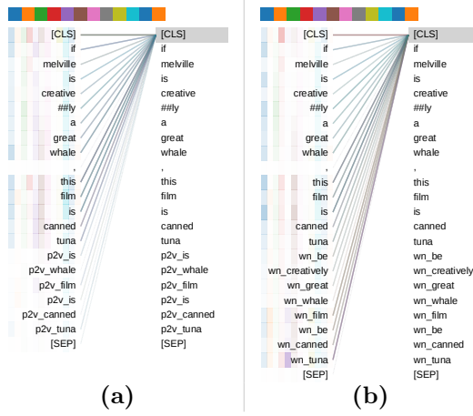
Figure 6: P2V-BERT and WN2V-BERT [CLS] token attention when a wrong output is given.
