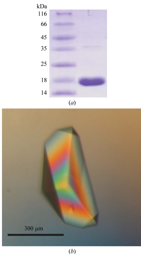
Figure 1 (a) SDS-PAGE (15%) of the TLDC domain after the last step of purification. 15 \mu\text{g} protein was loaded onto the gel. (b) TLDC-domain crystal.
