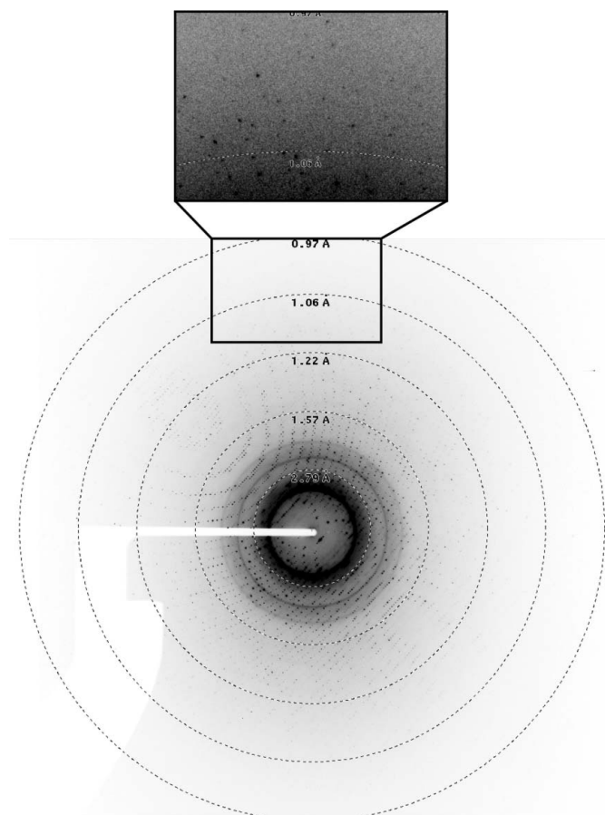
Figure 2 Diffraction image of a native TLDC crystal. The enlargement shows diffraction spots extending to 0.97 Å.
