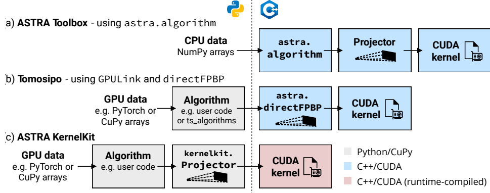
FIGURE 1. Software overview of ASTRA Toolbox, Tomosipo [23], and ASTRA KernelKit, illustrating where its components are located with respect to the Python-C++ language barrier. (a) and (b) show two methods of accessing a projector in ASTRA Toolbox. In comparison, the new ASTRA KernelKit uses a Python-based projector, as well as run-time compilation of the CUDA kernel. The figure is further explained in Section 3.1.
