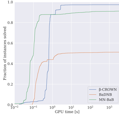
(c) GPU - MNIST
