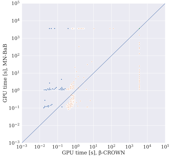
(c) GPU - MNIST
