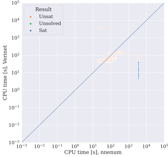
(a) CPU - MNIST
