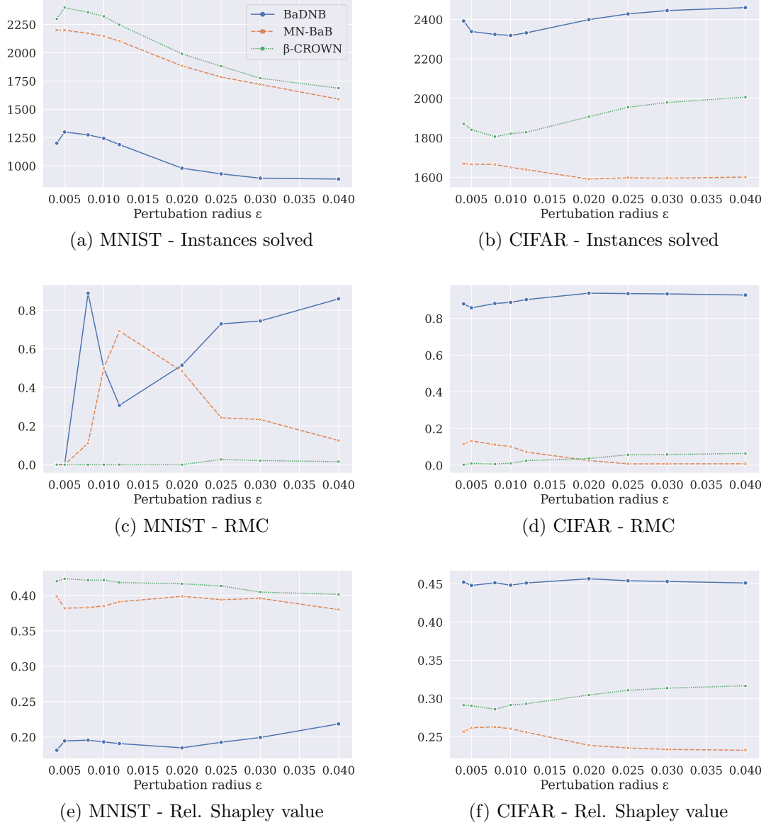
Figure 6: Performance of GPU-based verifiers for different values of \epsilon in the ReLU category.
