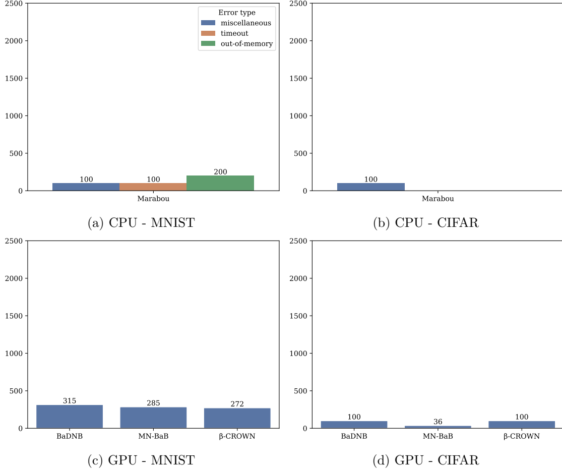
Figure C.1: Frequency of error types returned by the considered verification algorithms on instances in the ReLU+MaxPool category. The total number of instances in this category is 400 for MNIST and 100 for CIFAR.
