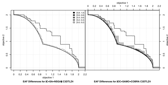
Fig. A.12. EAF difference plot C3DTLZ4.
