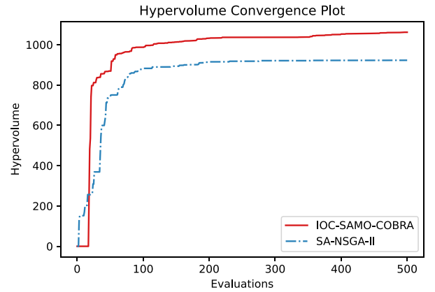
Fig. 8. Comparison of the hypervolume maximization progress between IOC-SAMO-COBRA and SA-NSGA-II ( p = 3 , each) on the ship design problem. x-axis: Number of function evaluations; y-axis: Hypervolume.
