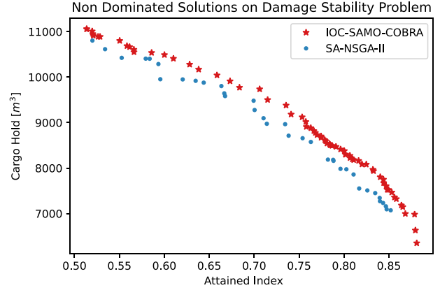
Fig. 7. Comparison of Pareto fronts obtained by IOC-SAMO-COBRA and SA-NSGA-II ( p = 3 , each) on the ship design problem. x-axis: Survivability index; y-axis: Cargo hold (both \uparrow max).
