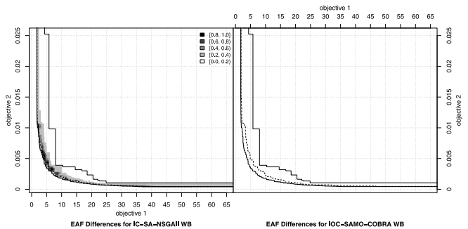
Fig. A.26. EAF difference plot WB.
