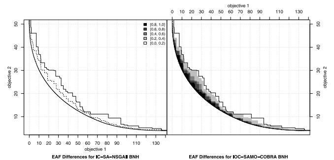
Fig. A.11. EAF difference plot BNH.
