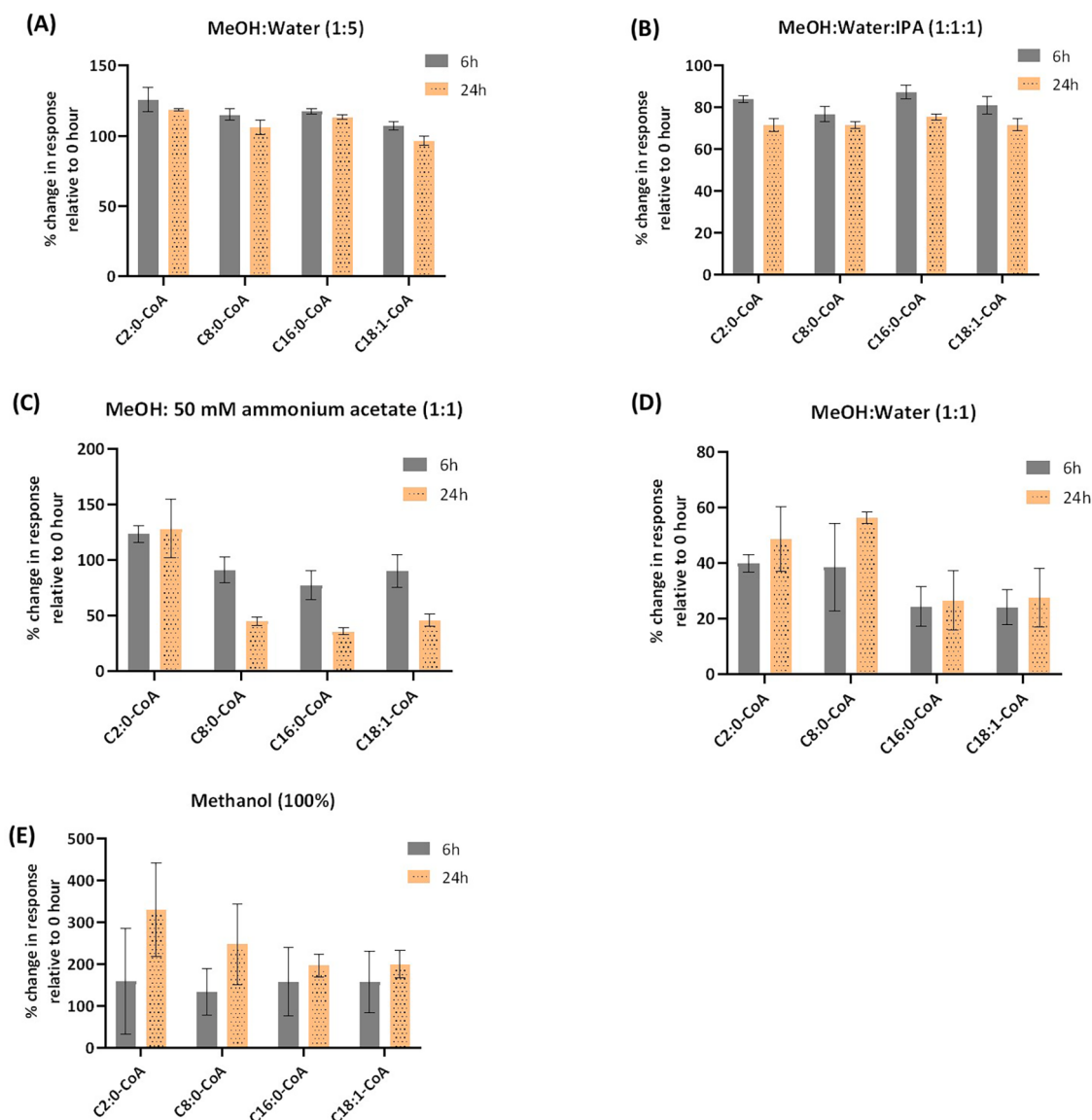
Fig. 3. Stability of representative acyl-CoA standards (C2:0 CoA, C8:0 CoA, C16:0 CoA and C18:1 CoA) in different injections solvents. (A) MeOH:Water (1:5,v/v); (B) MeOH:Water:IPA (1:1:1,v/v/v); (C) MeOH:50 mM ammonium acetate (1:1,v/v); (D) MeOH:Water (1:1,v/v); (E) Methanol (100%).
