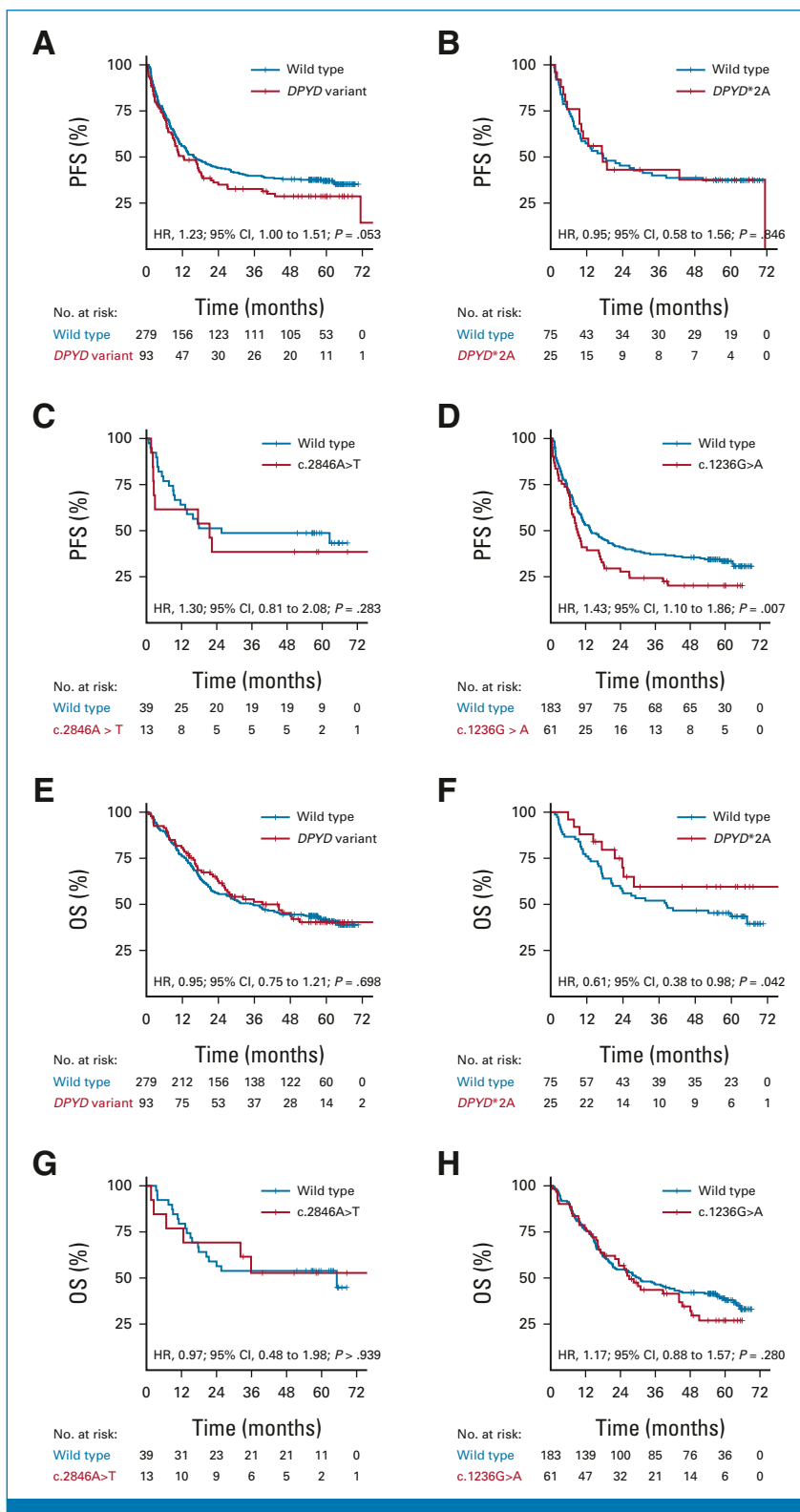
FIG 2. Kaplan-Meier plots and HRs for PFS and OS of pooled (A and E) DPYD variant carriers, (B and F) DPYD*2A , (C and G) c.2846A>T , and (D and H) c.1236G>A carriers. All P values indicated on the Kaplan-Meier curves were adjusted P values corresponding to the Cox regression analysis using the jackknife sandwich estimator. Censoring is indicated by tick marks. HRs, hazard ratios; OS, overall survival; PFS, progression-free survival.
