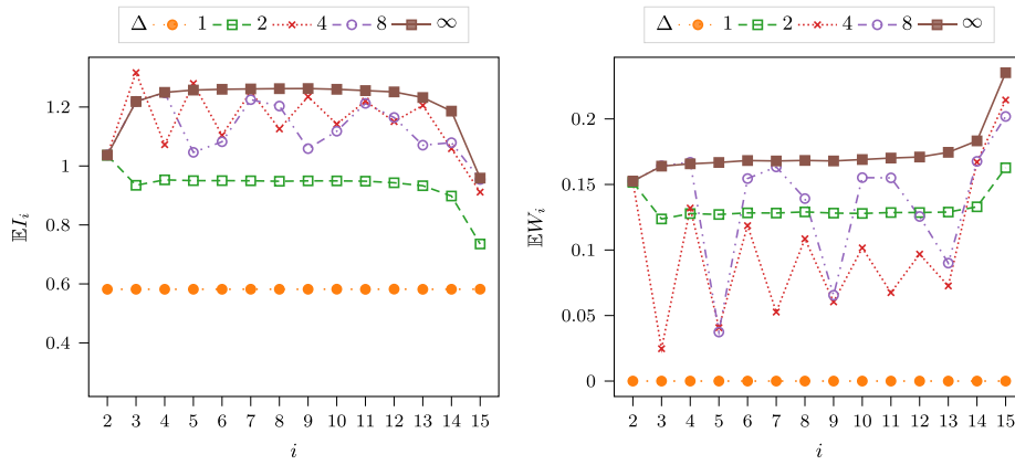
Fig. 6. Mean idle and waiting time of each client i = 2, \dots, n for \omega = 0.2 , n = 15 , and different values of \Delta .
