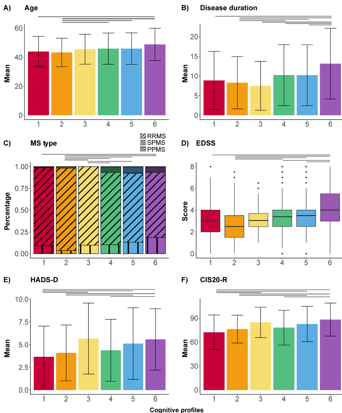
Fig. 3 Significant post hoc differences (indicated with a black stripe) between cognitive profiles (number on the x-axis) for age ( A ), disease duration ( B ), MS type ( C ), physical disability (EDSS; D ), symptoms of depression (HADS-D; E ), and level of fatigue (CIS20-R; F ). Abbreviations: RRMS relapsing–remitting MS, SPMS secondary pro-
