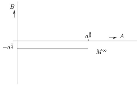
Fig. 3. A sketch of the manifold M^\infty in the A – B plane at \xi = \xi_{\max} .
