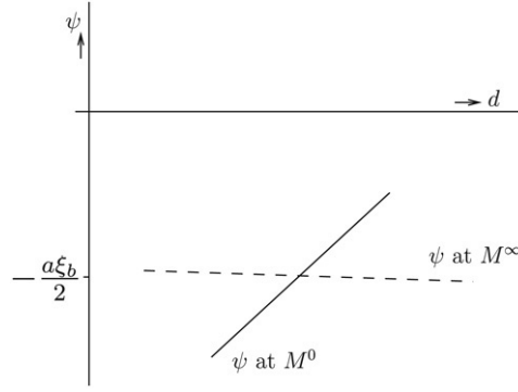
Fig. 10. A sketch of the \psi coordinates of the manifolds M^0 (solid curve) and M^\infty (dashed curve) at \xi = \xi_{\max} as a function of d .
