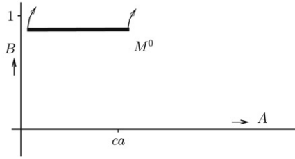
Fig. 4. A sketch of the manifold M^0 in the A – B plane at \xi = \xi_b .
