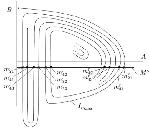
Fig. 8. A sketch of M^\infty and I_\eta at \eta = \eta_{\max} in the A – B plane. At the points marked by a cross, the m_{21}^r and m_{2i}^l , k = 2 solutions are formed for i = 1, 2, 3 . At the points marked by a dot, the m_{4i}^r and m_{4j}^l , k = 4 solutions occur for i, j = 1, 2, 3 . The existence of all of these intersection points is demonstrated in Section 6. Note that only some of the intersection points that form a k = 4 solution are sketched here, to maintain clarity in this figure.
