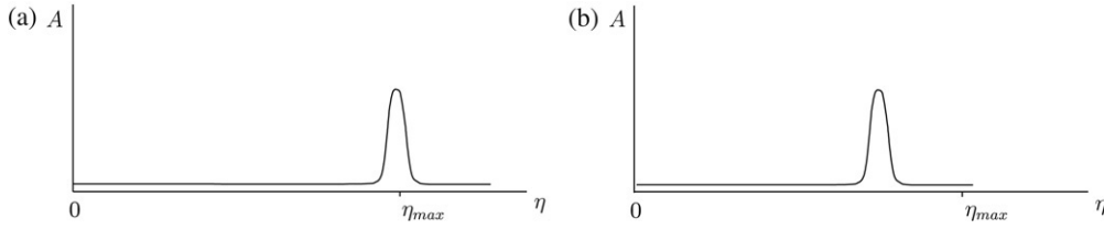
Fig. 9. A sketch of the different types of k = 2 solutions. (a) The solution of type R created at m_{21}^r . (b) The three solutions of type L , which are exponentially close to each other and hence indistinguishable in this sketch, correspond to the three intersection points m_{2i}^l , i = 1, 2, 3 .
