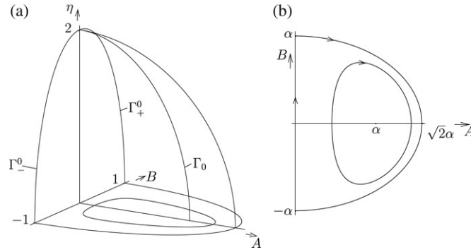
Fig. 5. (a) A sketch of the three curves of critical points \Gamma_{\pm}^0 and \Gamma_0 in the A – B – \eta plane for a = 0 . Here the positive B -axis points into the paper. (b) The flow in the A – B plane for \eta \in (\eta_{\min}, \eta_{\max}) fixed, where \alpha = \sqrt{1 - \frac{\eta^2}{4}} .
