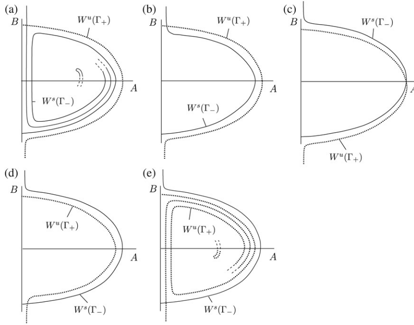
Fig. 6. A sequence of sketches of the manifolds W^u(\Gamma_+) (dotted curve) and W^s(\Gamma_-) (solid curve) in the A - B plane as \eta increases from \eta_{\min} to \eta_{\max} . Their positions are determined in Section 5. (a) At \eta = \eta_{\min} , W^s(\Gamma_-) is curled up inside W^u(\Gamma_+) and starts to pull back as \eta increases. As long as \eta_{\min} \leq \eta < \eta_{\text{zero}} , W^u(\Gamma_+) lies ‘outside’ W^s(\Gamma_-) at B = 0 . (b) The smaller the value of a , the more the tongue winds around the centre point, and hence in the sketch we only show the tip of the tongue and not all the spirals. (c) For \eta = \eta_{\text{zero}} , the two manifolds intersect at B = 0 . Increasing \eta further (d), W^u(\Gamma_+) starts to curl up inside W^s(\Gamma_-) up to \eta_{\max} (e) where for \eta_{\text{zero}} \leq \eta < \eta_{\max} , W^u(\Gamma_+) lies ‘inside’ W^s(\Gamma_-) at B = 0 .
