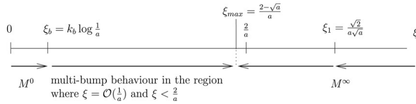
Fig. 2. The different points and intervals on the \xi -axis. As explained in Section 2, solutions on the manifolds M^\infty and M^0 are tracked to \xi_{\max} from \infty and 0, respectively, and it is shown that these manifolds have two families of transverse intersection points at \xi_{\max} . The multi-bump, self-similar, blow-up solutions of Theorem 2.1 are found in these transverse intersections.
