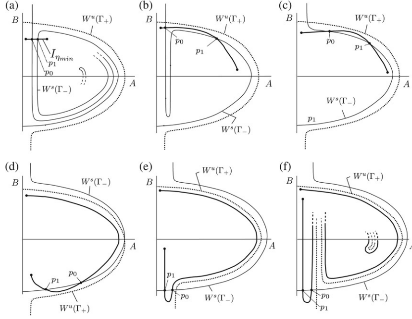
Fig. 7. The transformation of I_\eta as \eta is increased from \eta_{\min} to \eta_{\max} . During this process the point p_0 remains on W^u(\Gamma_+) , and the point p_1 remains on W^s(\Gamma_-) . (a) At \eta = \eta_{\min} , I_\eta is an interval approximately perpendicular to the B -axis. The smaller the value of a , the more the tongue winds around the centre point, and hence in the sketch we only denote the tip of the tongue and not all the spirals. ((b)–(d)) A – B planes at different values of \eta in Step I. I_\eta curls up as W^u(\Gamma_+) pulls back, where frame (d) is a sketch for \eta = \eta_{\text{zero}} . ((e), (f)) In step II, W^u(\Gamma_+) curls up in itself like a tongue. (f) At \eta = \eta_{\max} , I_\eta has formed a tongue structure as a result of the fact that W^u(\Gamma_+) curls up.
