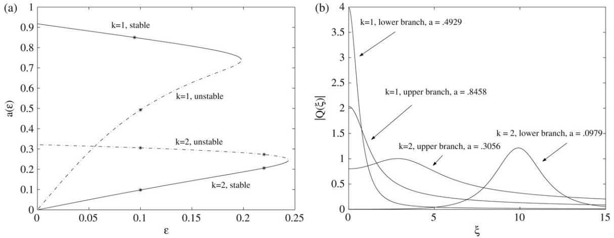
Fig. 1. (a) The k = 1 solution branch, the solutions with one maximum on (-\infty, \infty) , and the k = 2 solution branch, the solutions with two maxima on (-\infty, \infty) , plotted in the (\varepsilon, a) -plane where d = 3 and b = 0 . In (b), the solutions corresponding to the *'s are given. (b) Final-time profiles where the amplitude |Q| is plotted as a function of the spatial variable \xi for \varepsilon = 0.1 . The solutions correspond to the *'s in (a). This is a reproduction of Figs. 1.1 and 1.2 in [6].
