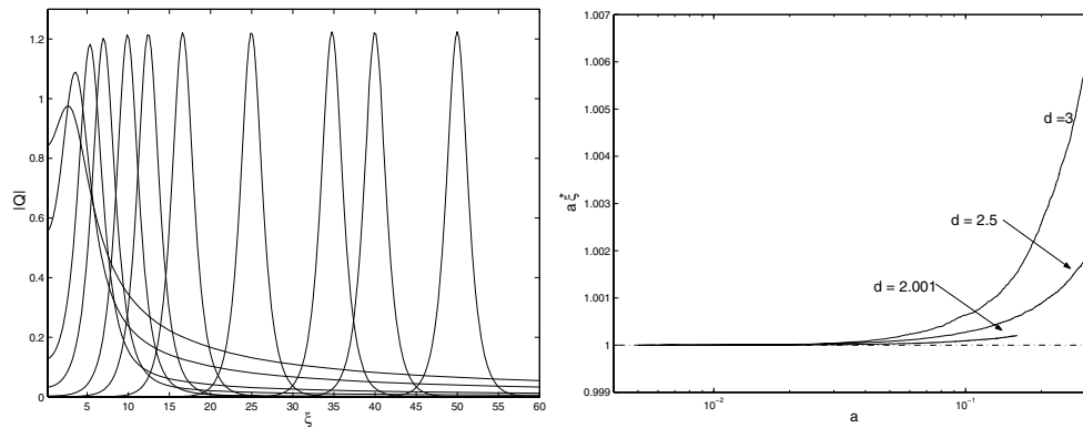
Figure 5. Left: The amplitude of the solutions |Q_2(\xi)| for \xi > 0 as a and \varepsilon are moving along the (k=2) -solution branch for d=3 . The peak of the solution moves to the right as a is decreased to zero. For smaller values of a , the solutions have a similar form and the peak \xi^* is located close to \frac{1}{a} . Right: The location of the maximum \xi^* along the (k=2) -solution branch for various choices of d where a\xi^* is plotted as a function of a .
