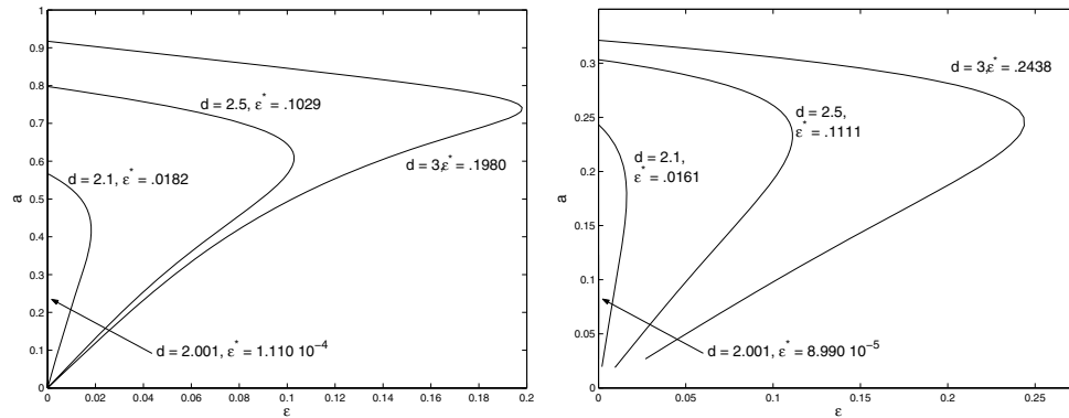
Figure 4. Left: The (k=1) -solution branch. The monotone solution is found here, in the (\varepsilon, a) -plane for different choices of d where \delta = 0 . Right: The (k=2) -solution branch. The solution Q_2 with two maxima on the real line is found here, in the (\varepsilon, a) -plane for different choices of d where \delta = 0 . The value of the fold bifurcation point \varepsilon_k^*(d) is also given for the branches.
