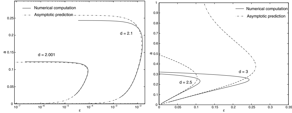
Figure 6. Comparison of the numerical results (solid line) and the asymptotic expansion for a_- and a_+ (dashed line) of the (k = 2) -solution branch. Left: Here d = 2.1, 2.001 and \varepsilon is plotted on a log-scale. Right: For d = 2.5 and d = 3 .
