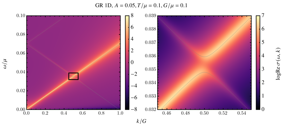
Figure 8: (Left) \text{Re } \sigma(\omega, k) plotted in the (k/G, \omega/\mu) plane for A = 0.05, T/\mu = 0.1 and G/\mu = 0.1 . (Right) Zoom on the Brillouin zone boundary at k = G/2 (region indicated by a black frame from on the left-hand plot) showing the level repulsion and the gapped sound mode at the edge of the zone. The gray dots are the hydrodynamic prediction given by numerically finding the roots of the determinant of Eq. (43).
