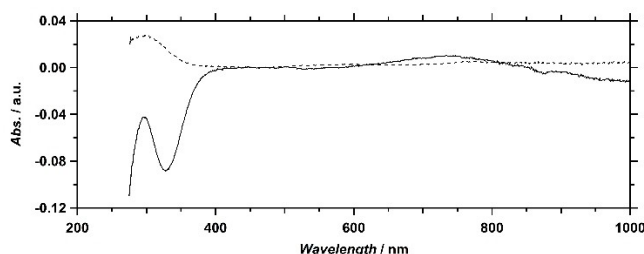
Figure 10. Difference spectrum after addition of \text{HNET}_3\text{PF}_6 (black trace) to the electrolyte solution containing 0.3 mM Cu-tmpa and 100 mM \text{NBu}_4\text{PF}_6 in MeCN, and between the start at t=0 min, and the end at t=360 min (dashed trace).
