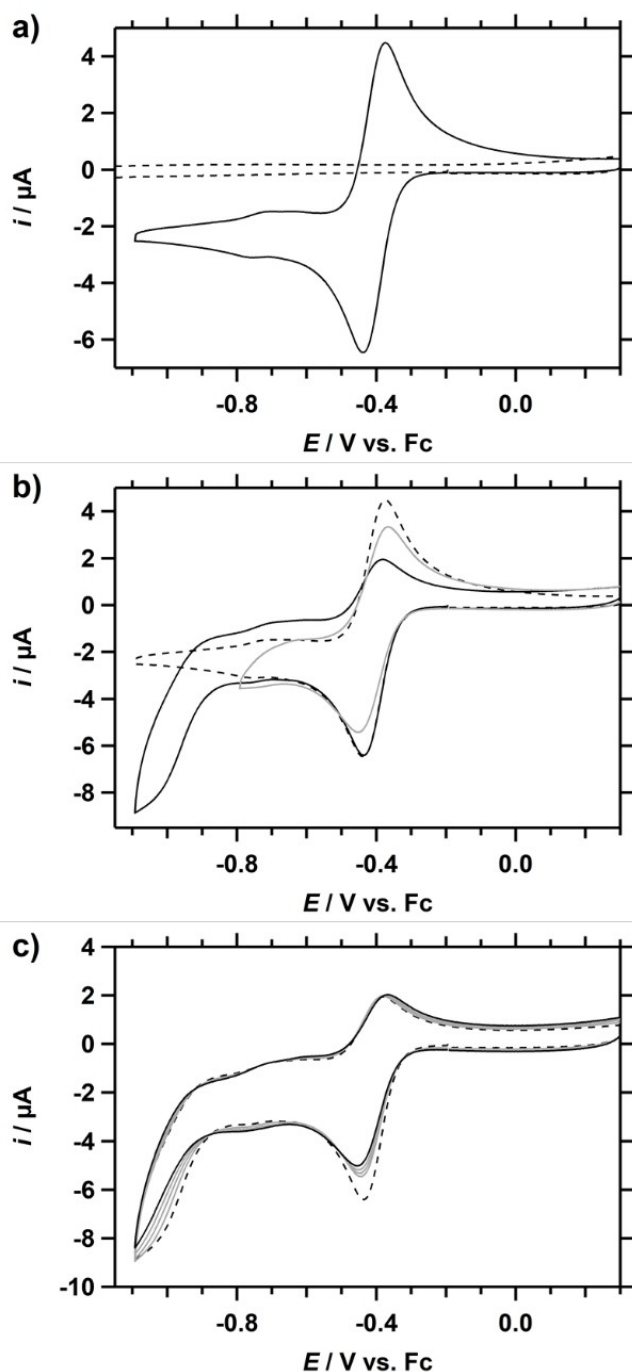
Figure 1. a) Cyclic voltammogram of Cu-tmpa (0.3 mM) in the absence of acid, including GC blank measurement (dashed), under 1 atm Ar. b) CVs of Cu-tmpa in the presence of 1 atm \text{O}_2 with varying potential windows. The redox couple in the presence of Ar is shown for comparison (dashed). c) CVs showing the redox behavior in the presence of oxygen over 5 cycles; first scan (dashed trace) and last scan (solid trace). Conditions: \text{NBu}_4\text{PF}_6 (100 mM) in MeCN, 100 \text{ mV s}^{-1} , 293 K.
