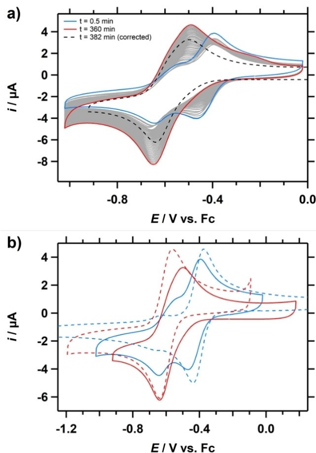
Figure 9. (a) CVs of Cu-tmpa (0.3 mM) in the presence of 50 mM \text{HNEt}_3\text{PF}_6 under 1 atm Ar, measured at 5 min time intervals after addition of the acid. (b) A comparison of CVs of 0.3 mM Cu-tmpa in the absence of acid (dashed blue trace), at t=0.5 \text{ min} after addition of 50 mM \text{HNEt}_3^+ (blue trace), at t=382 \text{ min} after addition of 50 mM \text{HNEt}_3^+ (red trace), and in a solution containing 100 mM \text{HNEt}_3^+ (dashed red trace). Conditions: \text{NBu}_4\text{PF}_6 (100 mM) in MeCN, 100 \text{ mVs}^{-1} , 293 K.
