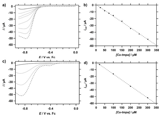
Figure 11. (a) Background-corrected LSVs of the catalytic ORR by Cu-tmpa in the presence of \text{HNET}_3\text{PF}_6 (50 mM) under 1 atm \text{O}_2 , for catalyst concentrations ranging from 25 (black) to 300 (dashed) \mu\text{M} . (b) Peak catalytic current i_{\text{cat}} at -0.78 V vs. Fc. (c) Background-corrected LSV of the catalytic ORR by Cu-tmpa in the presence of HOAc (100 mM) under 1 atm \text{O}_2 , for catalyst concentrations ranging from 20 to 300 \mu\text{M} . (d) Peak catalytic current i_{\text{cat}} at -0.85 V vs. Fc. Conditions: \text{NBu}_4\text{PF}_6 (100 mM) in MeCN, 100 \text{mV s}^{-1} , 293 K.
