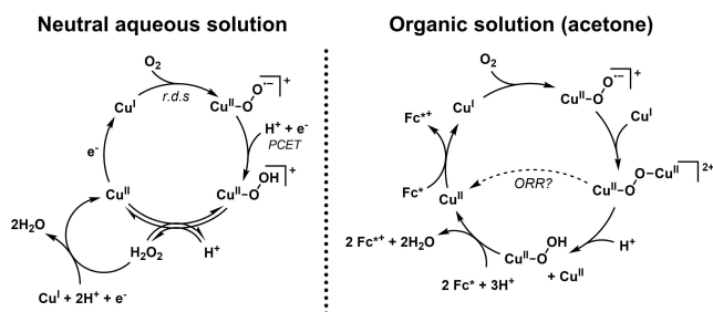
Scheme 1. Different catalytic mechanisms have been proposed for the reduction of \text{O}_2 by Cu-tmpa in neutral aqueous solution (electrochemistry driven), [5d] and in acetone (ferrocene-mediated). [5b,h,9c] The tmpa ligand is excluded from the scheme for clarity.
