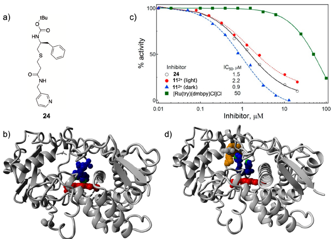
Figure 8. (a) Formula of the CYP3A4-inhibiting ritonavir analogue 24 photocaged by Turro et al. with the [\text{Ru}(\text{tpy})(\text{dmbpy})]^{2+} moiety. (b) X-ray structure of the uncaged CYP3A4 inhibitor shown in (a) bound via pyridine coordination to the heme iron center (PDB: 4D78). (c) Protein activity dose–response curves for the uncaged inhibitor 24 , the ruthenium-caged inhibitor 11 2+ (Figure 5) in the dark and after light activation, and the control ruthenium caging group [\text{Ru}(\text{tpy})(\text{dmbpy})\text{Cl}]\text{Cl} . (d) X-ray structure of the caged CYP3A4 inhibitor 11 2+ interacting with CYP3A4 without pyridine coordination to the heme iron center (PDB: 7KS8). Color code: pyridine nitrogen atoms are in green, heme is in red, the inhibitor 24 is in blue, and the ruthenium caging group of 11 2+ is in orange. Adapted from ref 80. Copyright 2021 American Chemical Society.
