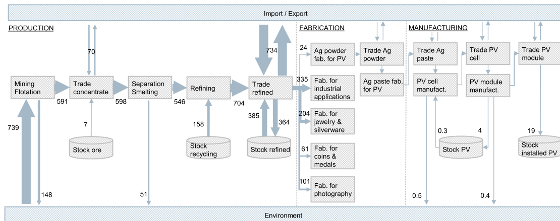
Fig. 2. Global silver flows cumulated over the period 1995-2021, in kilotons of silver. The width of the arrows is proportional to the magnitude of flows. Flows from and to the stocks of silver ore, refined silver, and manufactured cells and modules are derived from mass-balance at country-level. Trade flows from silver powder to PV module were calculated from a proportional trade distribution assumption and are therefore not detailed here.
