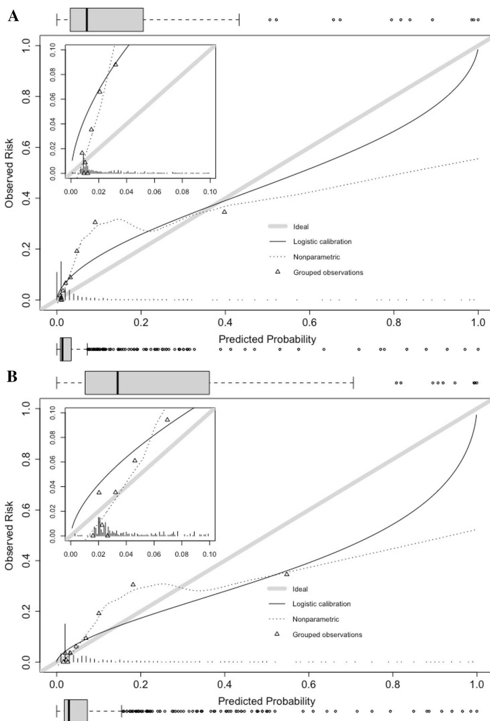
Fig. 2 Calibration plots (slope = 0.609) of the original Croce formula in the Dutch 2017 cohort (A) and after intercept recalibration (B; slope = 0.609); zoomed perspectives are included in the left upper corners. Box plots for probability distribution are added per calibration plot for patients with (upper) and without (lower) nosocomial pneumonia
